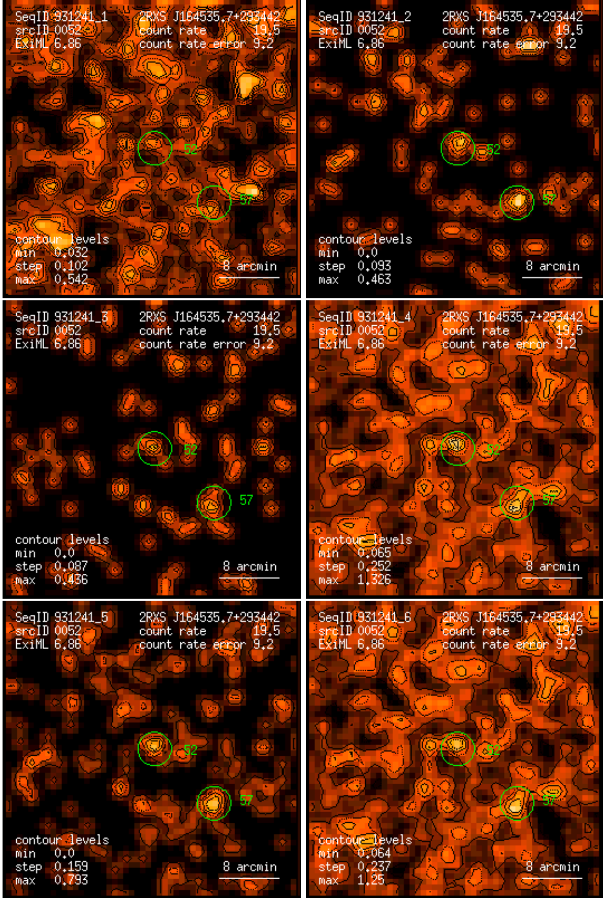
Figure 52: RASS 931241: detection 0052: band rate images, Gaussian filter: (1) PSPC channels 11 – 41, (2) 52 – 90, (3) 91 – 201, (4) 11 – 235, (5) 52 – 201, (6) 11 – 201. Broad band rates in counts/ks. Band rate contour levels in counts/ks/arcmin 2 .
