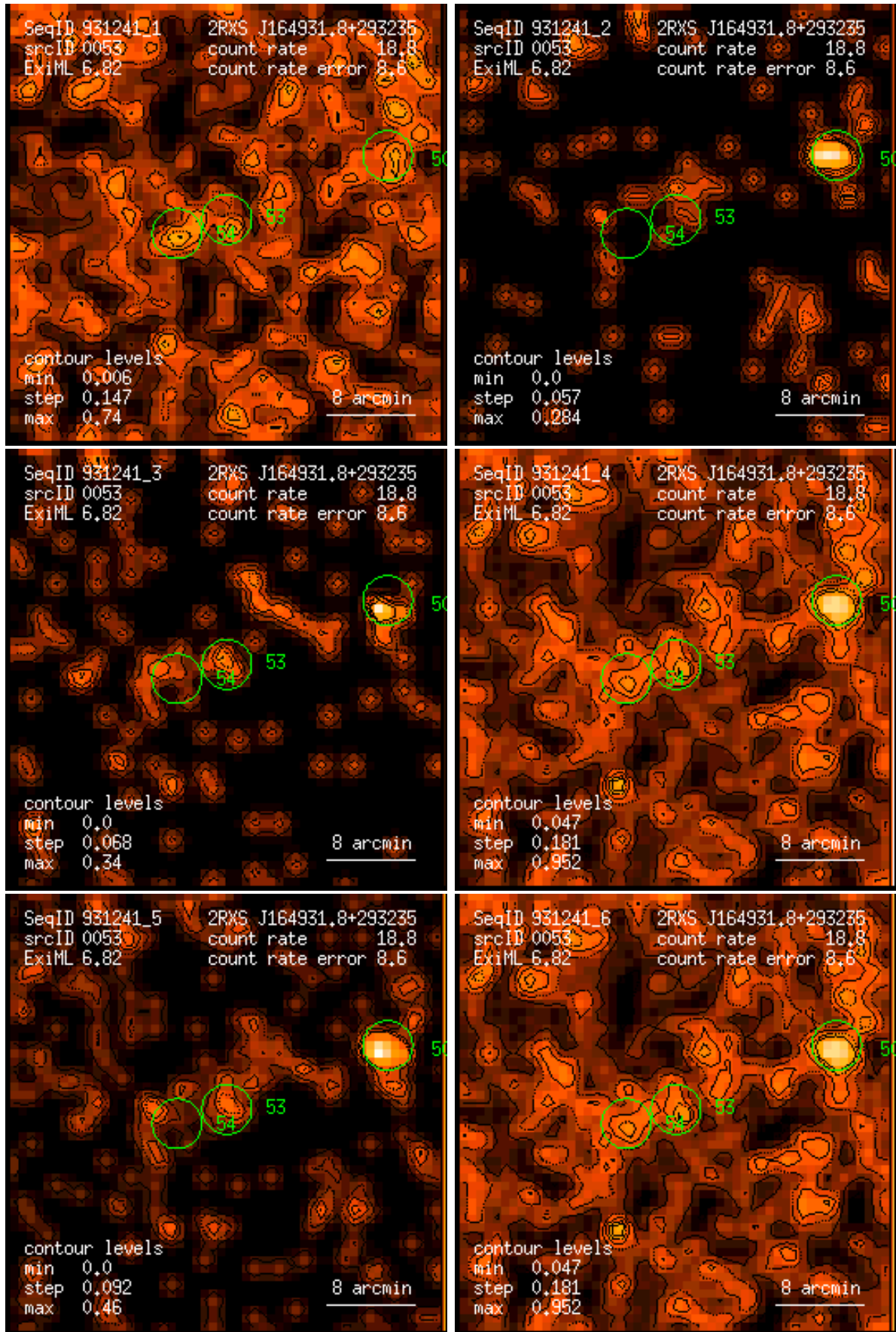
Figure 53: RASS 931241: detection 0053: band rate images, Gaussian filter: (1) PSPC channels 11 – 41, (2) 52 – 90, (3) 91 – 201, (4) 11 – 235, (5) 52 – 201, (6) 11 – 201. Broad band rates in counts/ks. Band rate contour levels in counts/ks/arcmin 2 .
