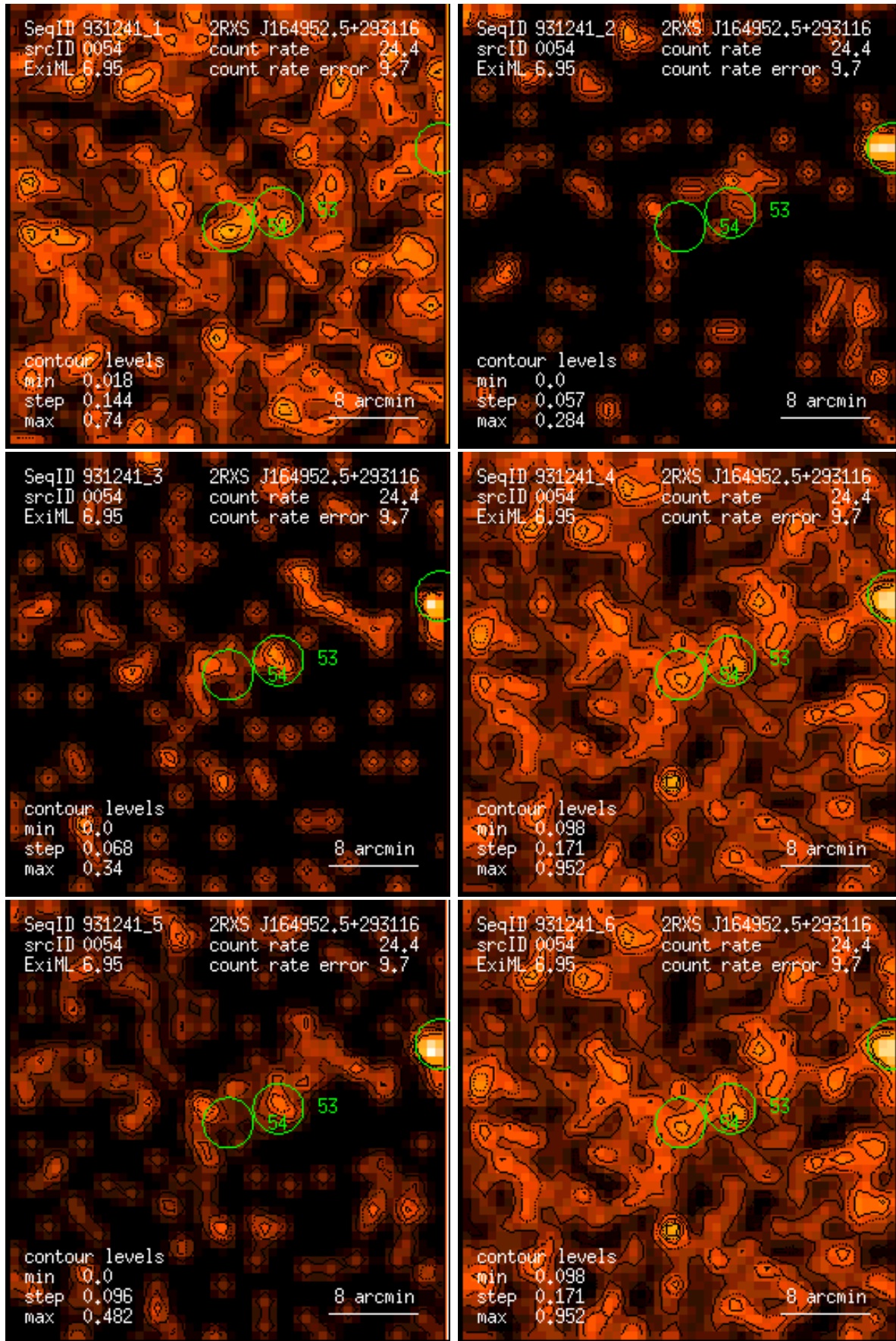
Figure 54: RASS 931241: detection 0054: band rate images, Gaussian filter: (1) PSPC channels 11 – 41, (2) 52 – 90, (3) 91 – 201, (4) 11 – 235, (5) 52 – 201, (6) 11 – 201. Broad band rates in counts/ks. Band rate contour levels in counts/ks/arcmin 2 .
