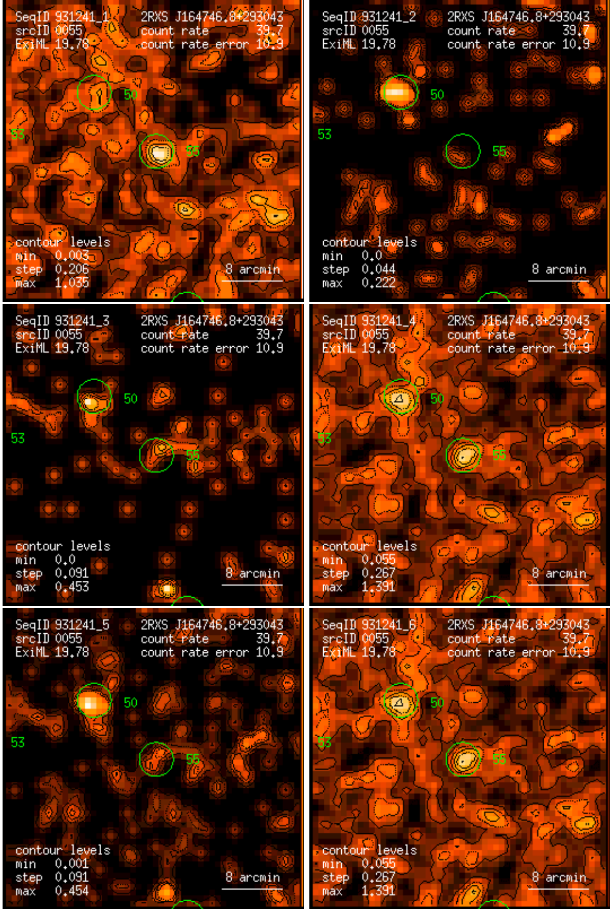
Figure 55: RASS 931241: detection 0055: band rate images, Gaussian filter: (1) PSPC channels 11 – 41, (2) 52 – 90, (3) 91 – 201, (4) 11 – 235, (5) 52 – 201, (6) 11 – 201. Broad band rates in counts/ks. Band rate contour levels in counts/ks/arcmin 2 .
