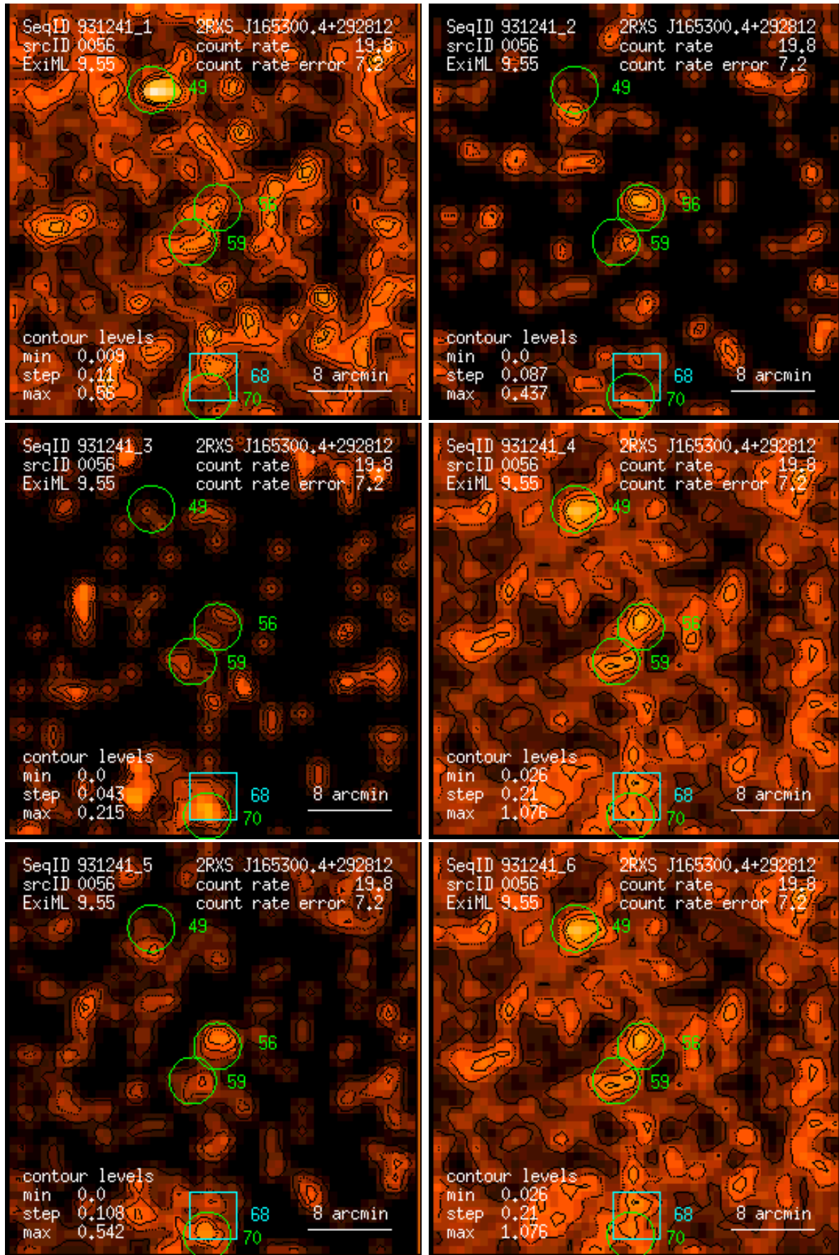
Figure 56: RASS 931241: detection 0056: band rate images, Gaussian filter: (1) PSPC channels 11 – 41, (2) 52 – 90, (3) 91 – 201, (4) 11 – 235, (5) 52 – 201, (6) 11 – 201. Broad band rates in counts/ks. Band rate contour levels in counts/ks/arcmin 2 .
