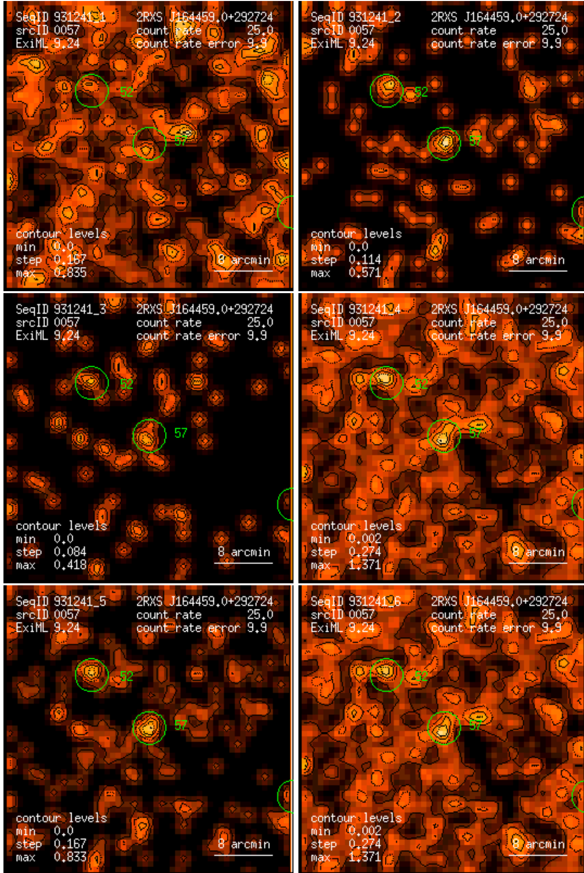
Figure 57: RASS 931241: detection 0057: band rate images, Gaussian filter: (1) PSPC channels 11 – 41, (2) 52 – 90, (3) 91 – 201, (4) 11 – 235, (5) 52 – 201, (6) 11 – 201. Broad band rates in counts/ks. Band rate contour levels in counts/ks/arcmin 2 .
