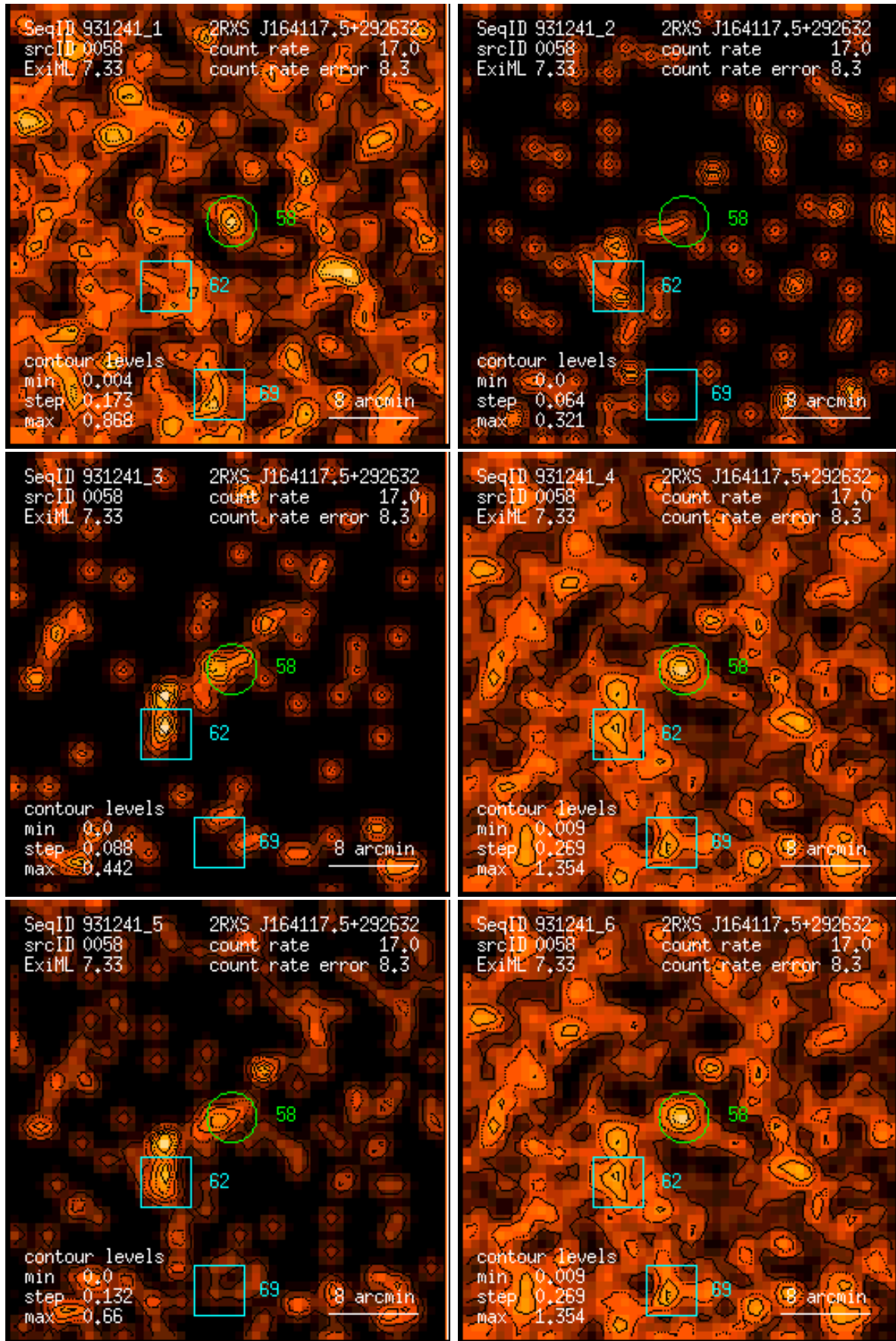
Figure 58: RASS 931241: detection 0058: band rate images, Gaussian filter: (1) PSPC channels 11 – 41, (2) 52 – 90, (3) 91 – 201, (4) 11 – 235, (5) 52 – 201, (6) 11 – 201. Broad band rates in counts/ks. Band rate contour levels in counts/ks/arcmin 2 .
