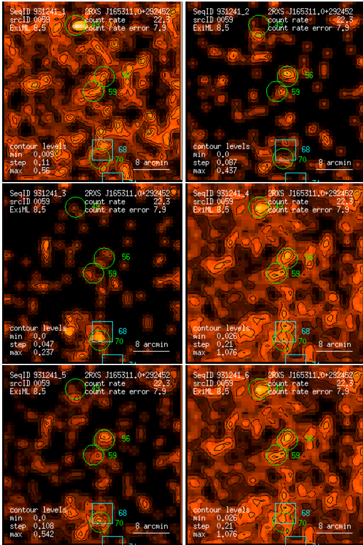
Figure 59: RASS 931241: detection 0059: band rate images, Gaussian filter: (1) PSPC channels 11 – 41, (2) 52 – 90, (3) 91 – 201, (4) 11 – 235, (5) 52 – 201, (6) 11 – 201. Broad band rates in counts/ks. Band rate contour levels in counts/ks/arcmin 2 .
