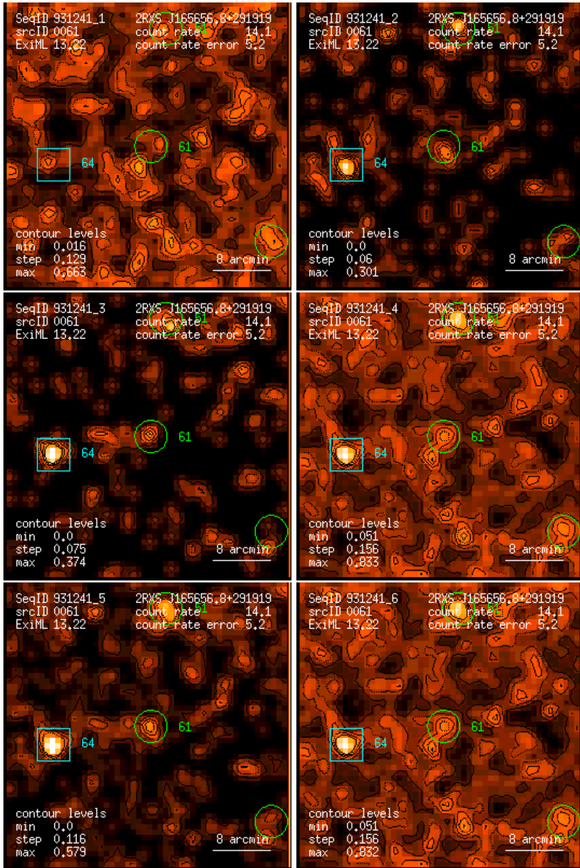
Figure 61: RASS 931241: detection 0061: band rate images, Gaussian filter: (1) PSPC channels 11 – 41, (2) 52 – 90, (3) 91 – 201, (4) 11 – 235, (5) 52 – 201, (6) 11 – 201. Broad band rates in counts/ks. Band rate contour levels in counts/ks/arcmin 2 .
