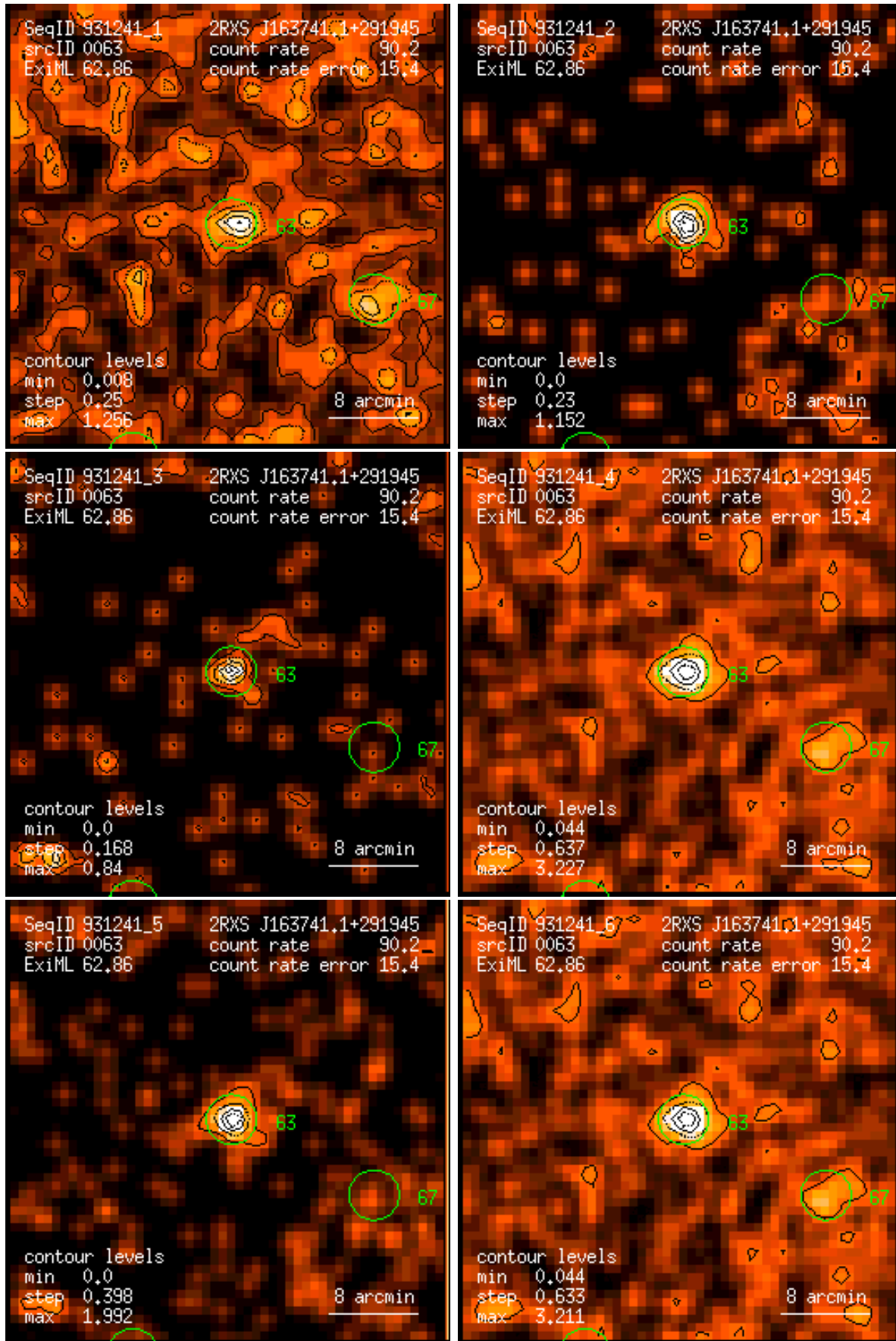
Figure 63: RASS 931241: detection 0063: band rate images, Gaussian filter: (1) PSPC channels 11 – 41, (2) 52 – 90, (3) 91 – 201, (4) 11 – 235, (5) 52 – 201, (6) 11 – 201. Broad band rates in counts/ks. Band rate contour levels in counts/ks/arcmin 2 .
