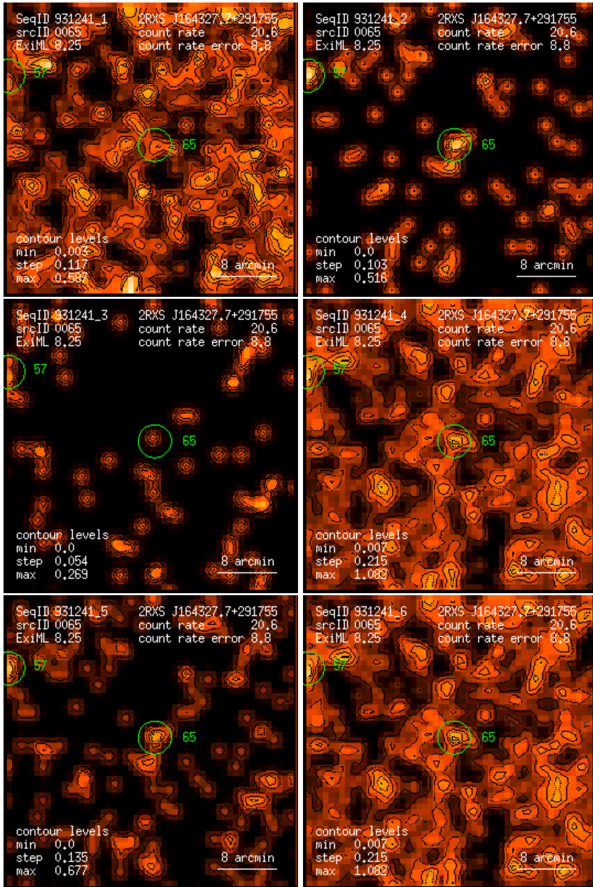
Figure 65: RASS 931241: detection 0065: band rate images, Gaussian filter: (1) PSPC channels 11 – 41, (2) 52 – 90, (3) 91 – 201, (4) 11 – 235, (5) 52 – 201, (6) 11 – 201. Broad band rates in counts/ks. Band rate contour levels in counts/ks/arcmin 2 .
