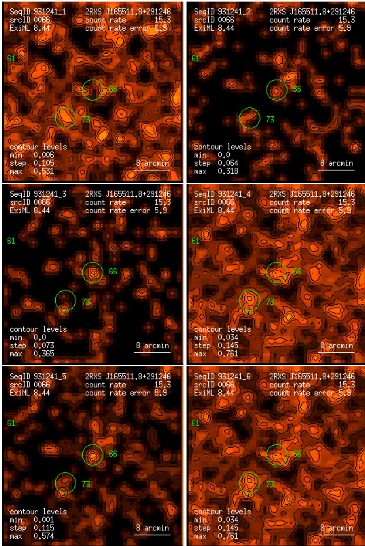
Figure 66: RASS 931241: detection 0066: band rate images, Gaussian filter: (1) PSPC channels 11 – 41, (2) 52 – 90, (3) 91 – 201, (4) 11 – 235, (5) 52 – 201, (6) 11 – 201. Broad band rates in counts/ks. Band rate contour levels in counts/ks/arcmin 2 .
