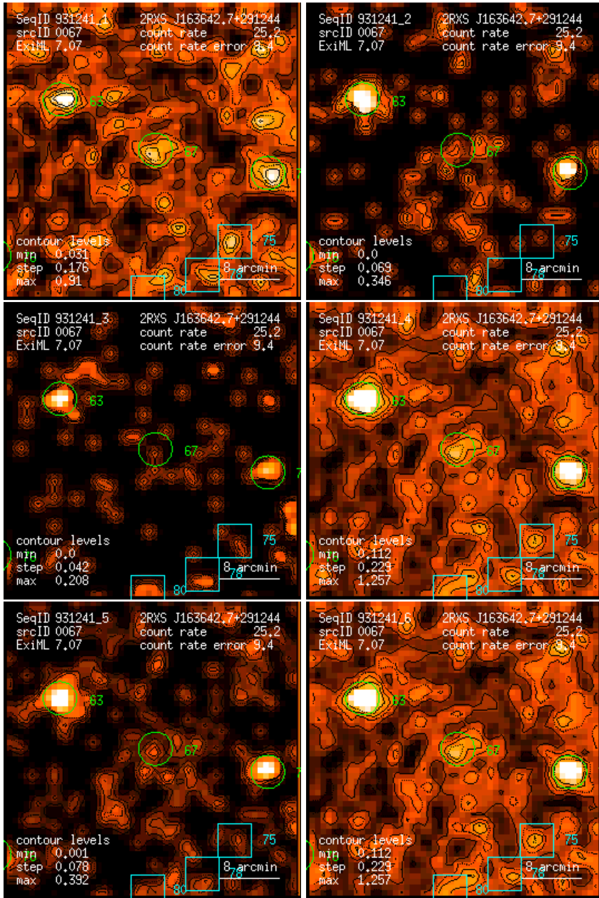
Figure 67: RASS 931241: detection 0067: band rate images, Gaussian filter: (1) PSPC channels 11 – 41, (2) 52 – 90, (3) 91 – 201, (4) 11 – 235, (5) 52 – 201, (6) 11 – 201. Broad band rates in counts/ks. Band rate contour levels in counts/ks/arcmin 2 .
