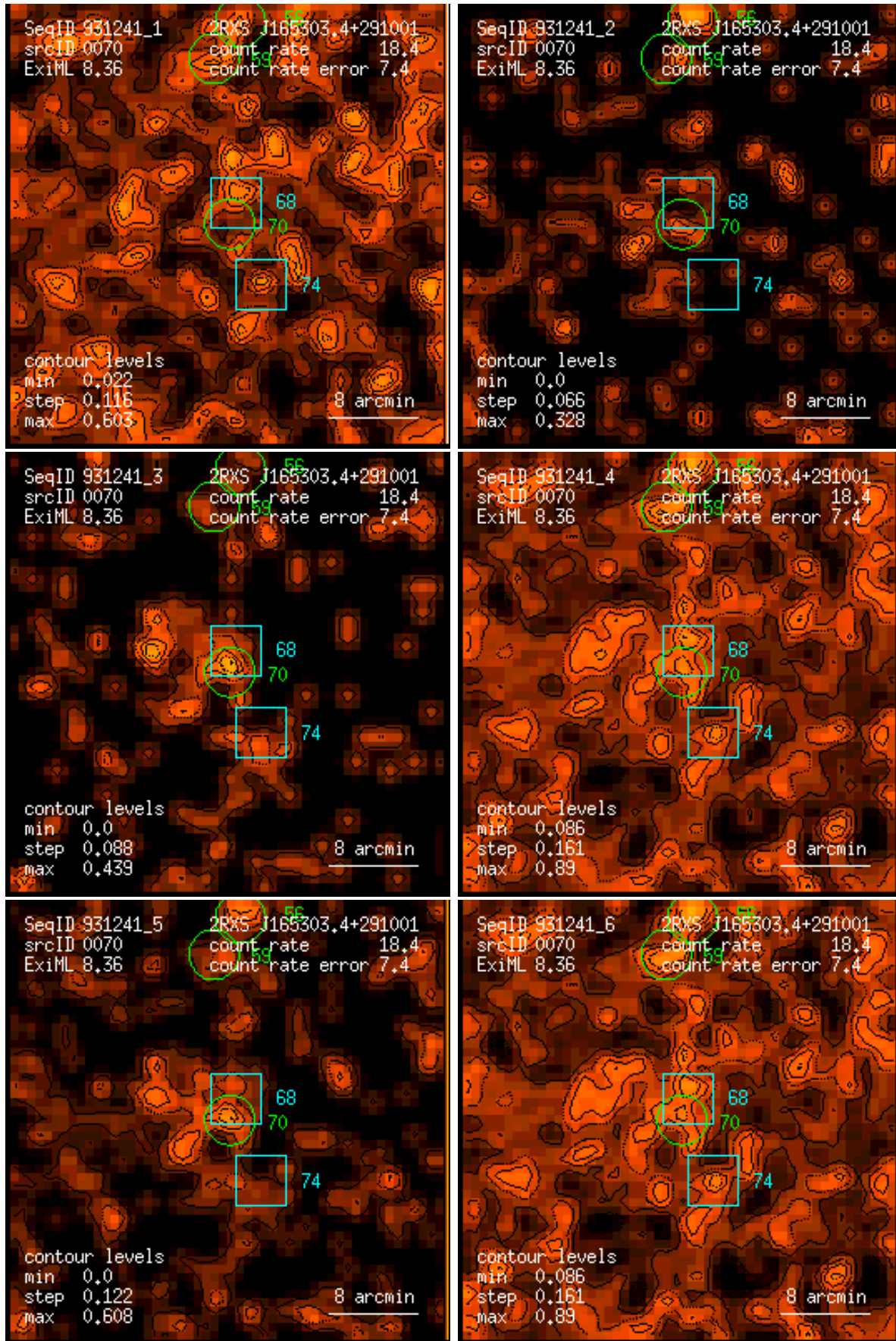
Figure 70: RASS 931241: detection 0070: band rate images, Gaussian filter: (1) PSPC channels 11 – 41, (2) 52 – 90, (3) 91 – 201, (4) 11 – 235, (5) 52 – 201, (6) 11 – 201. Broad band rates in counts/ks. Band rate contour levels in counts/ks/arcmin 2 .
