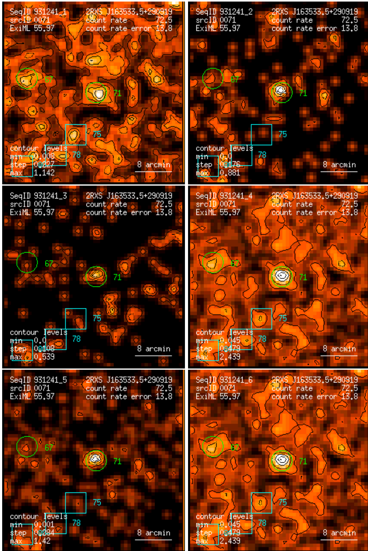
Figure 71: RASS 931241: detection 0071: band rate images, Gaussian filter: (1) PSPC channels 11 – 41, (2) 52 – 90, (3) 91 – 201, (4) 11 – 235, (5) 52 – 201, (6) 11 – 201. Broad band rates in counts/ks. Band rate contour levels in counts/ks/arcmin 2 .
