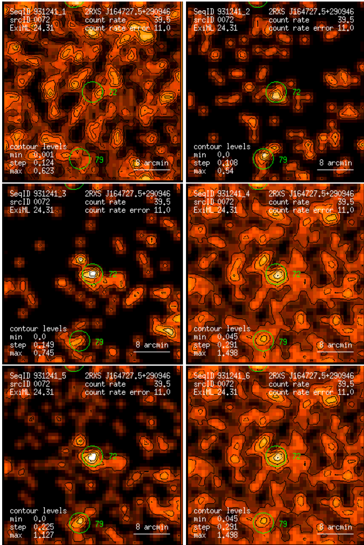
Figure 72: RASS 931241: detection 0072: band rate images, Gaussian filter: (1) PSPC channels 11 – 41, (2) 52 – 90, (3) 91 – 201, (4) 11 – 235, (5) 52 – 201, (6) 11 – 201. Broad band rates in counts/ks. Band rate contour levels in counts/ks/arcmin 2 .
