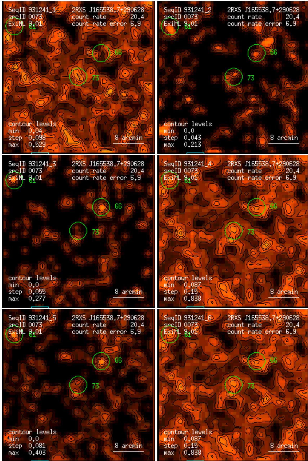
Figure 73: RASS 931241: detection 0073: band rate images, Gaussian filter: (1) PSPC channels 11 – 41, (2) 52 – 90, (3) 91 – 201, (4) 11 – 235, (5) 52 – 201, (6) 11 – 201. Broad band rates in counts/ks. Band rate contour levels in counts/ks/arcmin 2 .
