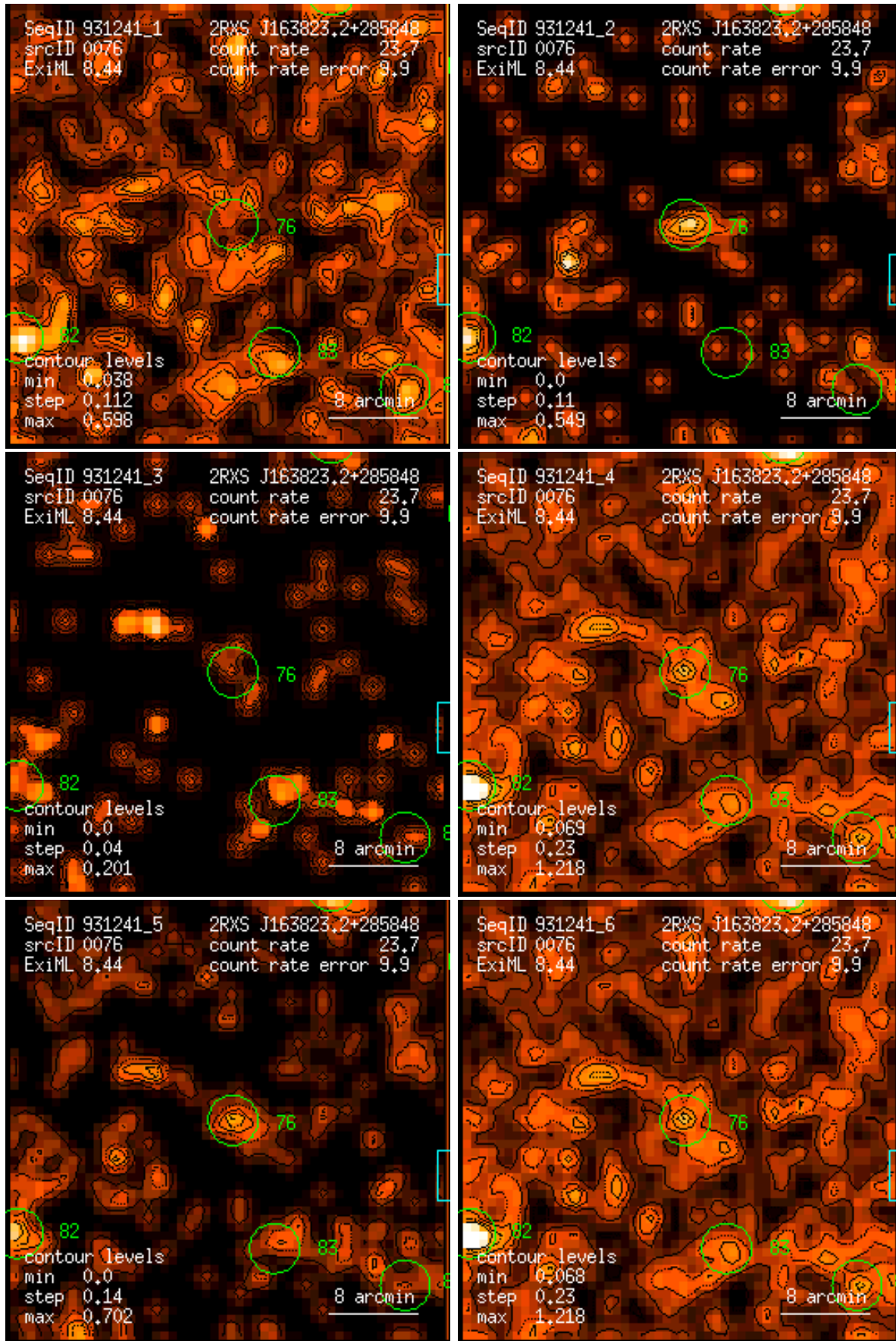
Figure 76: RASS 931241: detection 0076: band rate images, Gaussian filter: (1) PSPC channels 11 – 41, (2) 52 – 90, (3) 91 – 201, (4) 11 – 235, (5) 52 – 201, (6) 11 – 201. Broad band rates in counts/ks. Band rate contour levels in counts/ks/arcmin 2 .
