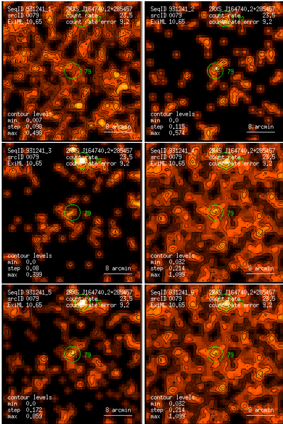
Figure 79: RASS 931241: detection 0079: band rate images, Gaussian filter: (1) PSPC channels 11 – 41, (2) 52 – 90, (3) 91 – 201, (4) 11 – 235, (5) 52 – 201, (6) 11 – 201. Broad band rates in counts/ks. Band rate contour levels in counts/ks/arcmin 2 .
