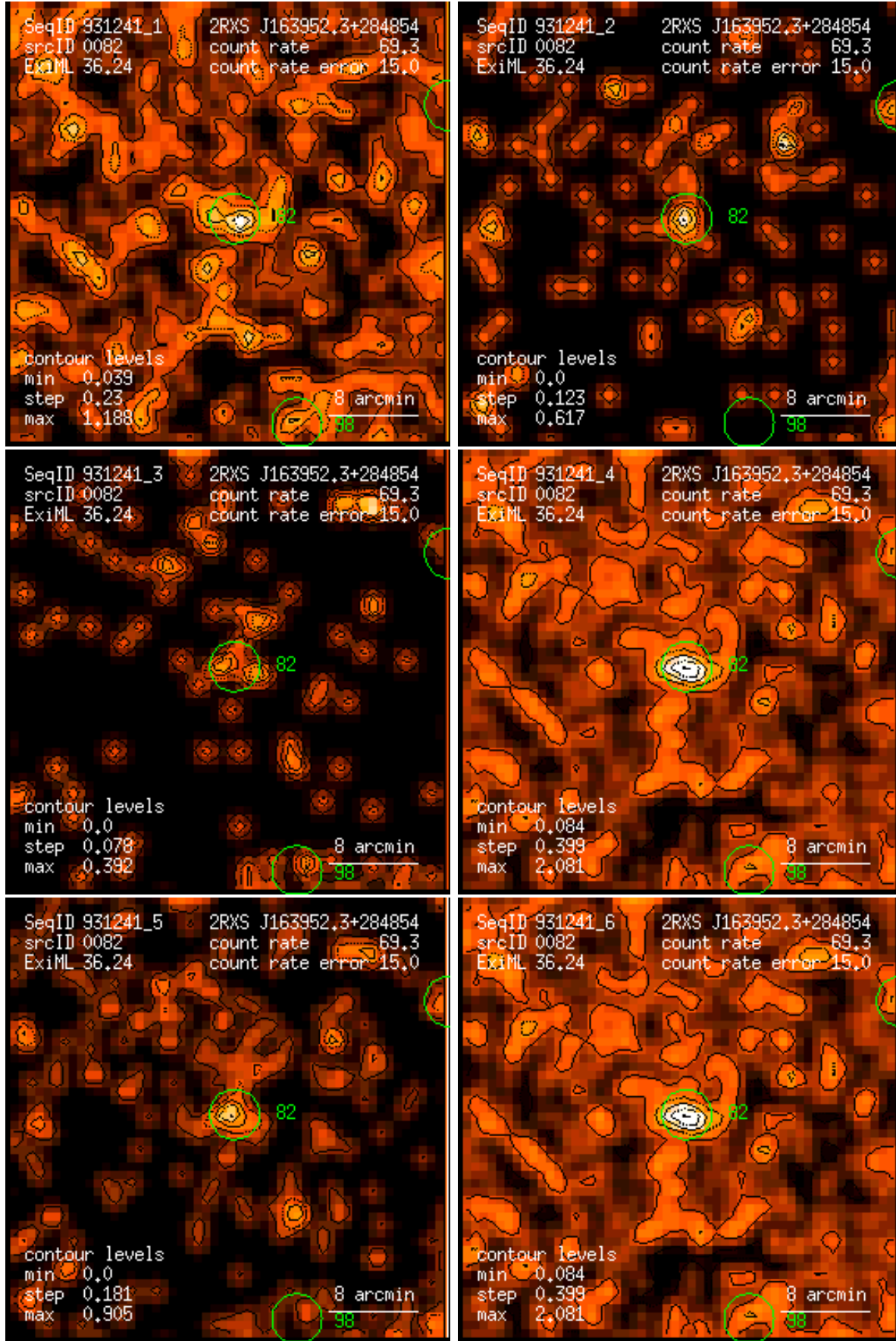
Figure 82: RASS 931241: detection 0082: band rate images, Gaussian filter: (1) PSPC channels 11 – 41, (2) 52 – 90, (3) 91 – 201, (4) 11 – 235, (5) 52 – 201, (6) 11 – 201. Broad band rates in counts/ks. Band rate contour levels in counts/ks/arcmin 2 .
