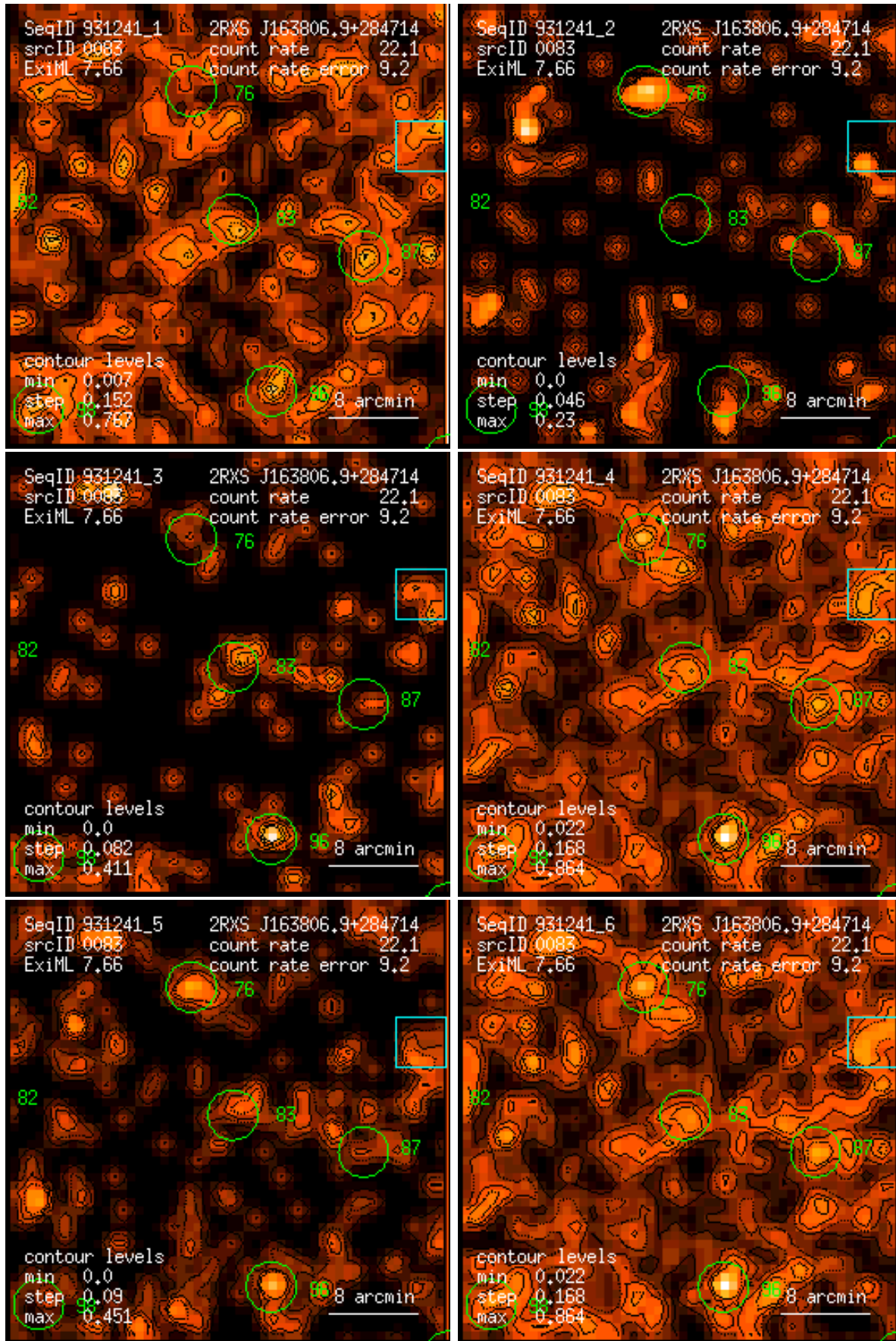
Figure 83: RASS 931241: detection 0083: band rate images, Gaussian filter: (1) PSPC channels 11 – 41, (2) 52 – 90, (3) 91 – 201, (4) 11 – 235, (5) 52 – 201, (6) 11 – 201. Broad band rates in counts/ks. Band rate contour levels in counts/ks/arcmin 2 .
