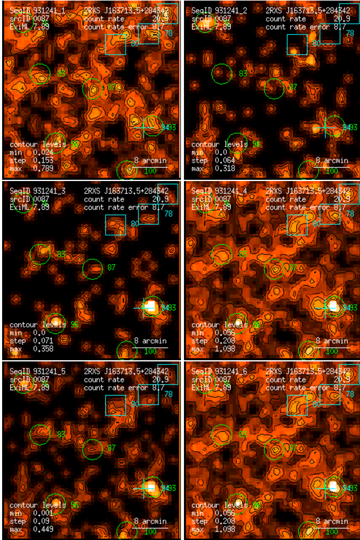
Figure 87: RASS 931241: detection 0087: band rate images, Gaussian filter: (1) PSPC channels 11 – 41, (2) 52 – 90, (3) 91 – 201, (4) 11 – 235, (5) 52 – 201, (6) 11 – 201. Broad band rates in counts/ks. Band rate contour levels in counts/ks/arcmin 2 .
