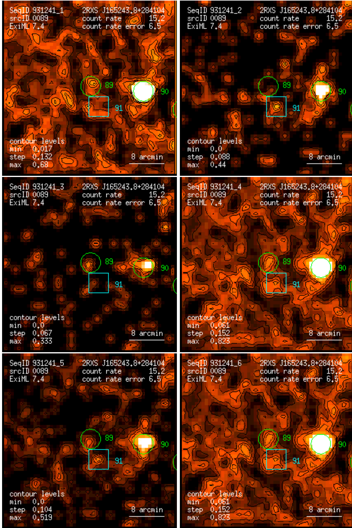
Figure 89: RASS 931241: detection 0089: band rate images, Gaussian filter: (1) PSPC channels 11 – 41, (2) 52 – 90, (3) 91 – 201, (4) 11 – 235, (5) 52 – 201, (6) 11 – 201. Broad band rates in counts/ks. Band rate contour levels in counts/ks/arcmin 2 .
