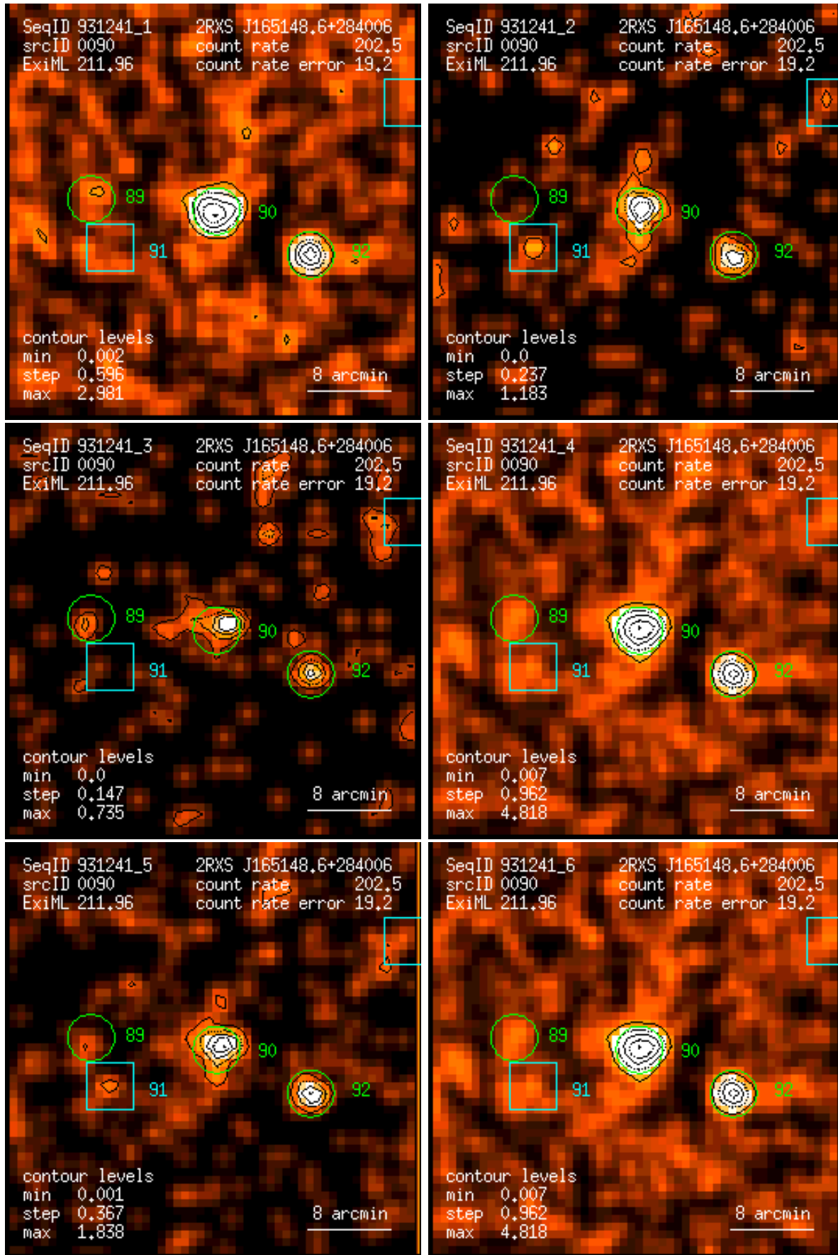
Figure 90: RASS 931241: detection 0090: band rate images, Gaussian filter: (1) PSPC channels 11 – 41, (2) 52 – 90, (3) 91 – 201, (4) 11 – 235, (5) 52 – 201, (6) 11 – 201. Broad band rates in counts/ks. Band rate contour levels in counts/ks/arcmin 2 .
