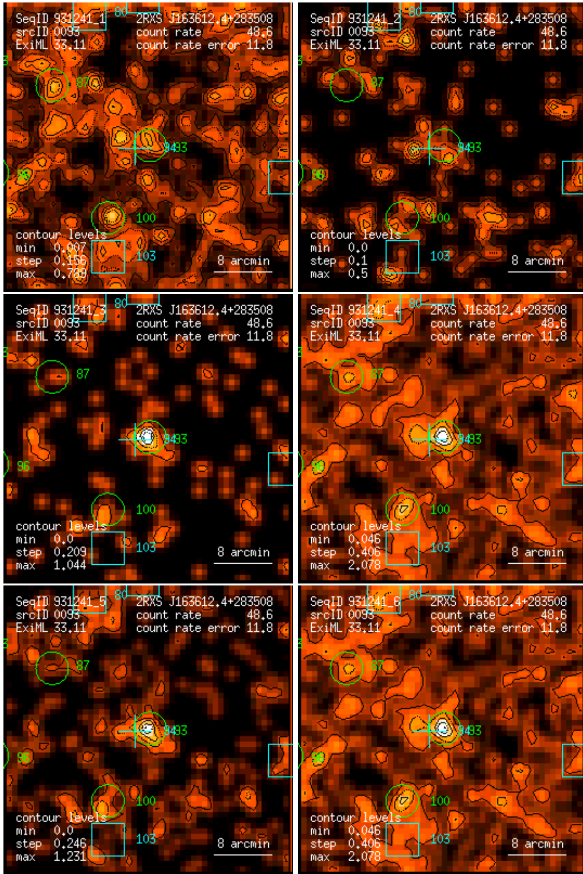
Figure 93: RASS 931241: detection 0093: band rate images, Gaussian filter: (1) PSPC channels 11 – 41, (2) 52 – 90, (3) 91 – 201, (4) 11 – 235, (5) 52 – 201, (6) 11 – 201. Broad band rates in counts/ks. Band rate contour levels in counts/ks/arcmin 2 .
