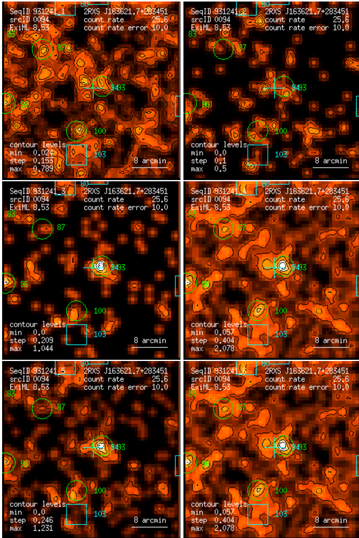
Figure 94: RASS 931241: detection 0094: band rate images, Gaussian filter: (1) PSPC channels 11 – 41, (2) 52 – 90, (3) 91 – 201, (4) 11 – 235, (5) 52 – 201, (6) 11 – 201. Broad band rates in counts/ks. Band rate contour levels in counts/ks/arcmin 2 .
