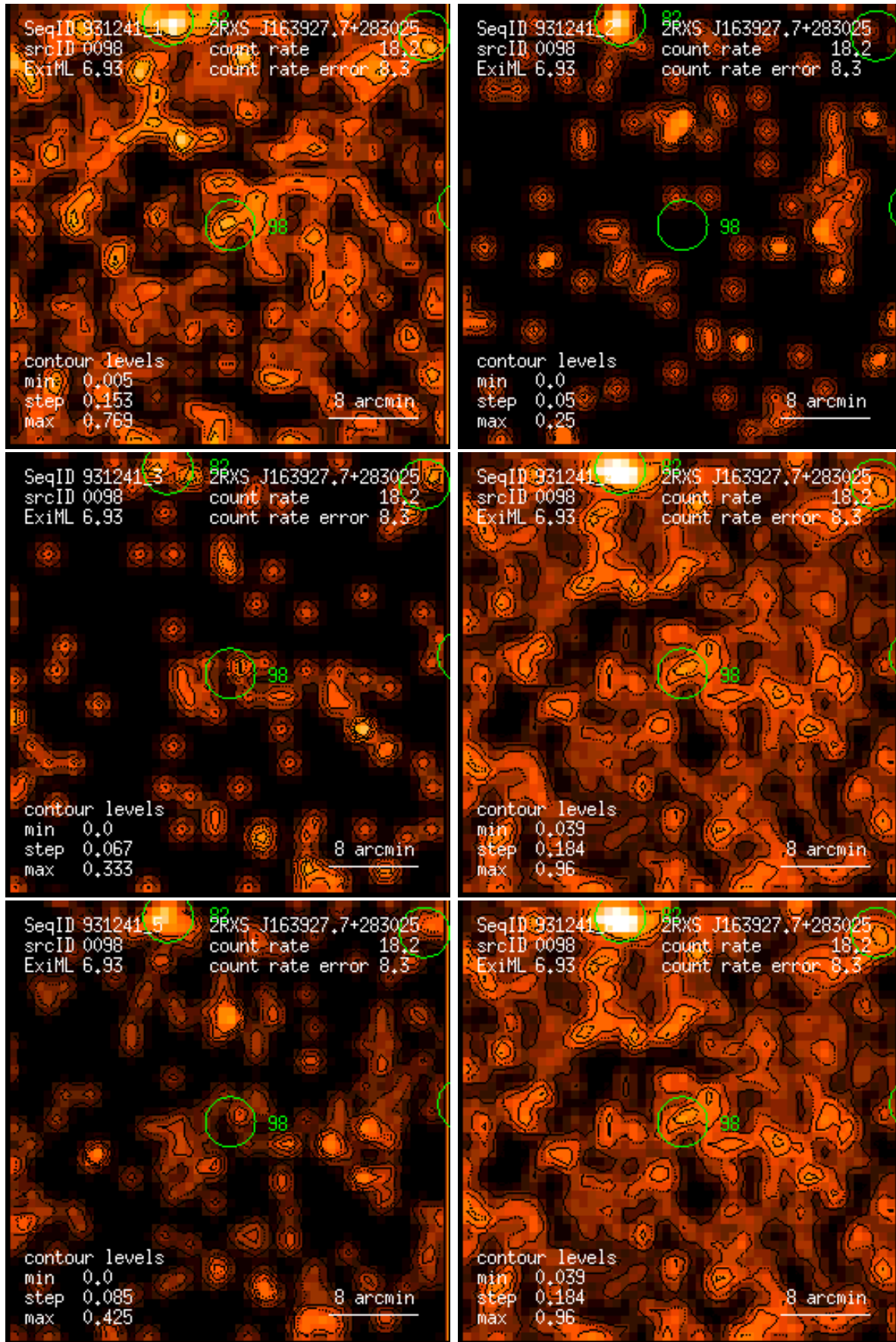
Figure 98: RASS 931241: detection 0098: band rate images, Gaussian filter: (1) PSPC channels 11 – 41, (2) 52 – 90, (3) 91 – 201, (4) 11 – 235, (5) 52 – 201, (6) 11 – 201. Broad band rates in counts/ks. Band rate contour levels in counts/ks/arcmin 2 .
