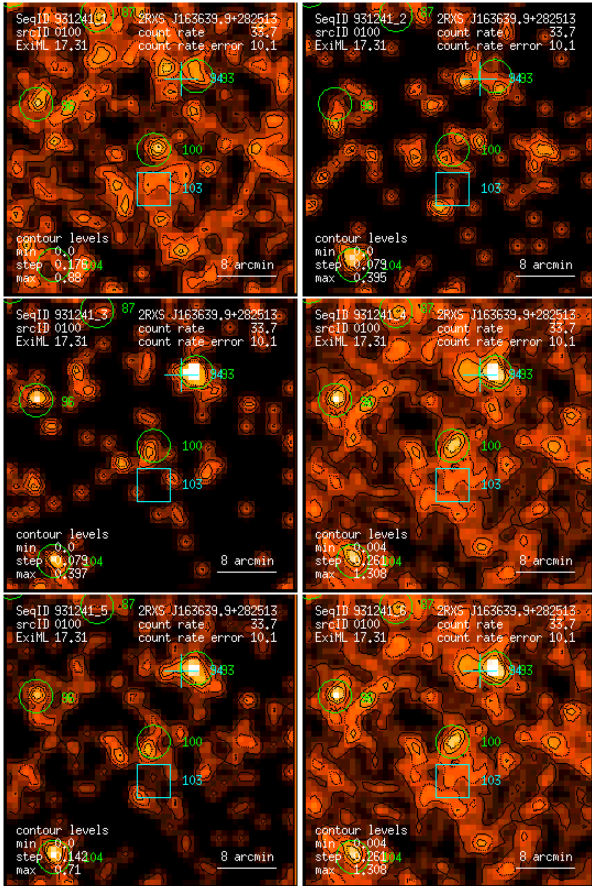
Figure 100: RASS 931241: detection 0100: band rate images, Gaussian filter: (1) PSPC channels 11 – 41, (2) 52 – 90, (3) 91 – 201, (4) 11 – 235, (5) 52 – 201, (6) 11 – 201. Broad band rates in counts/ks. Band rate contour levels in counts/ks/arcmin 2 .
