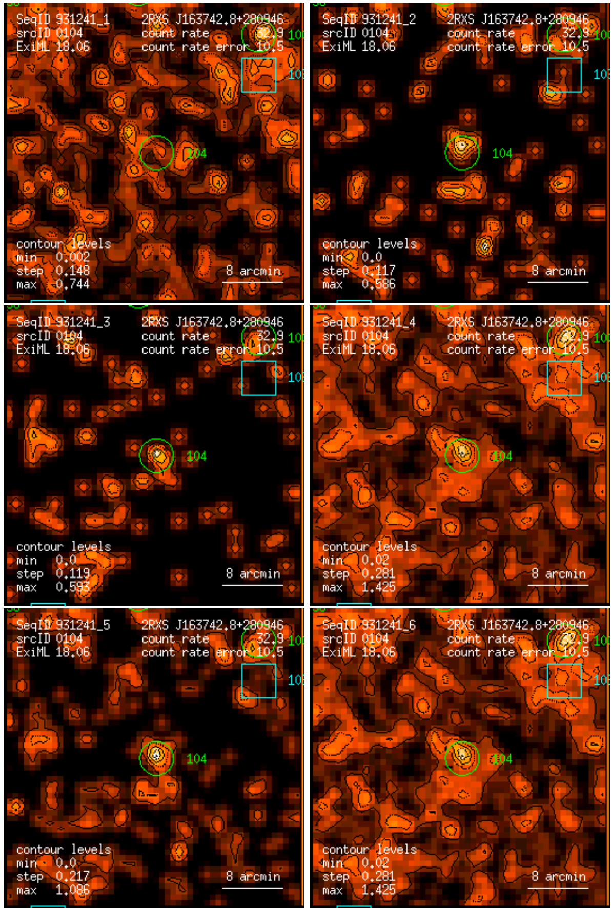
Figure 104: RASS 931241: detection 0104: band rate images, Gaussian filter: (1) PSPC channels 11 – 41, (2) 52 – 90, (3) 91 – 201, (4) 11 – 235, (5) 52 – 201, (6) 11 – 201. Broad band rates in counts/ks. Band rate contour levels in counts/ks/arcmin 2 .
