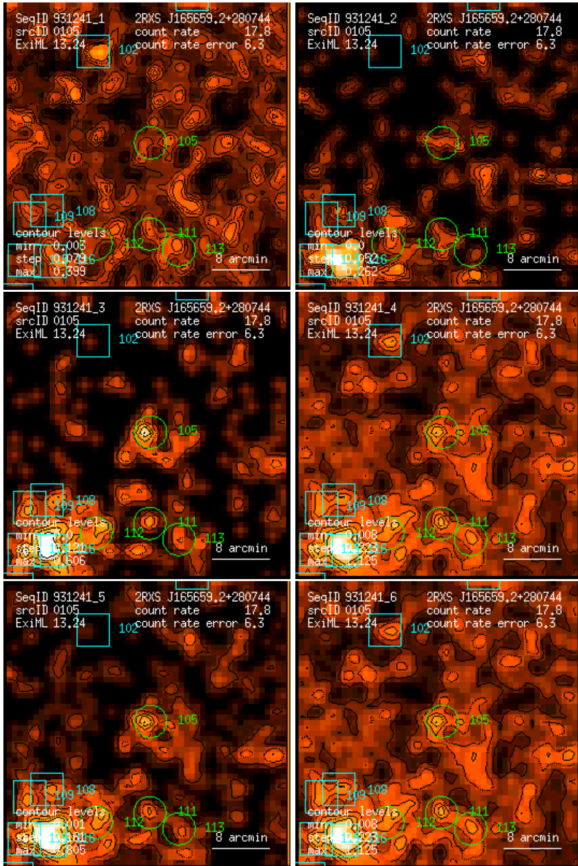
Figure 105: RASS 931241: detection 0105: band rate images, Gaussian filter: (1) PSPC channels 11 – 41, (2) 52 – 90, (3) 91 – 201, (4) 11 – 235, (5) 52 – 201, (6) 11 – 201. Broad band rates in counts/ks. Band rate contour levels in counts/ks/arcmin 2 .
