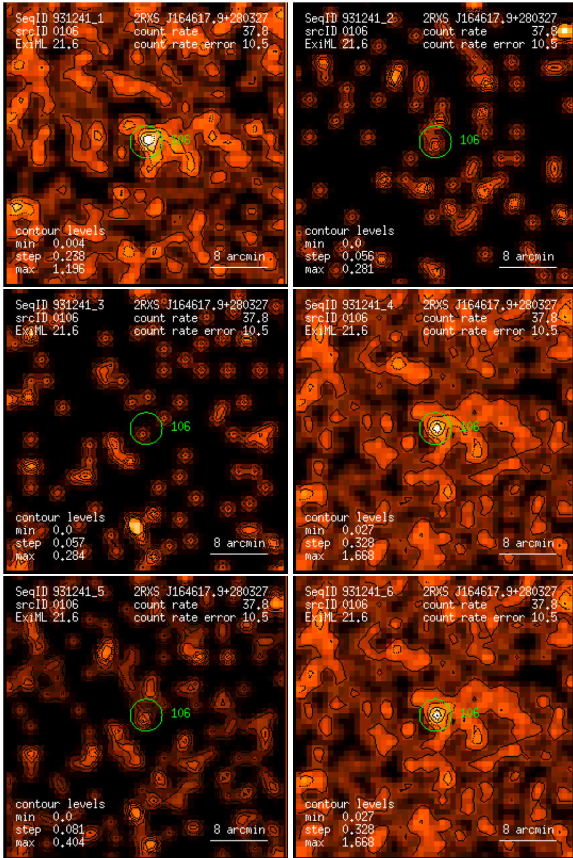
Figure 106: RASS 931241: detection 0106: band rate images, Gaussian filter: (1) PSPC channels 11 – 41, (2) 52 – 90, (3) 91 – 201, (4) 11 – 235, (5) 52 – 201, (6) 11 – 201. Broad band rates in counts/ks. Band rate contour levels in counts/ks/arcmin 2 .
