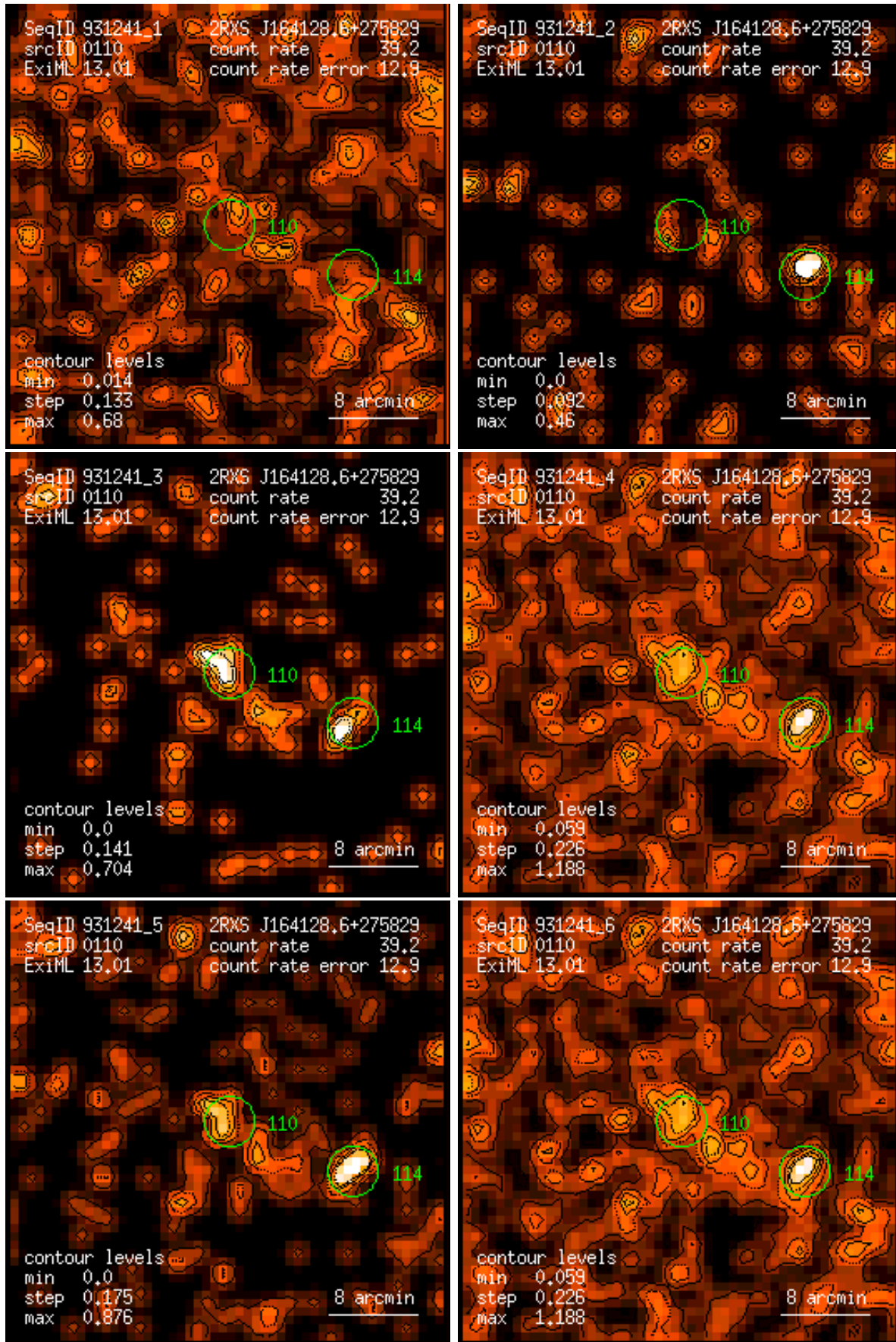
Figure 110: RASS 931241: detection 0110: band rate images, Gaussian filter: (1) PSPC channels 11 – 41, (2) 52 – 90, (3) 91 – 201, (4) 11 – 235, (5) 52 – 201, (6) 11 – 201. Broad band rates in counts/ks. Band rate contour levels in counts/ks/arcmin 2 .
