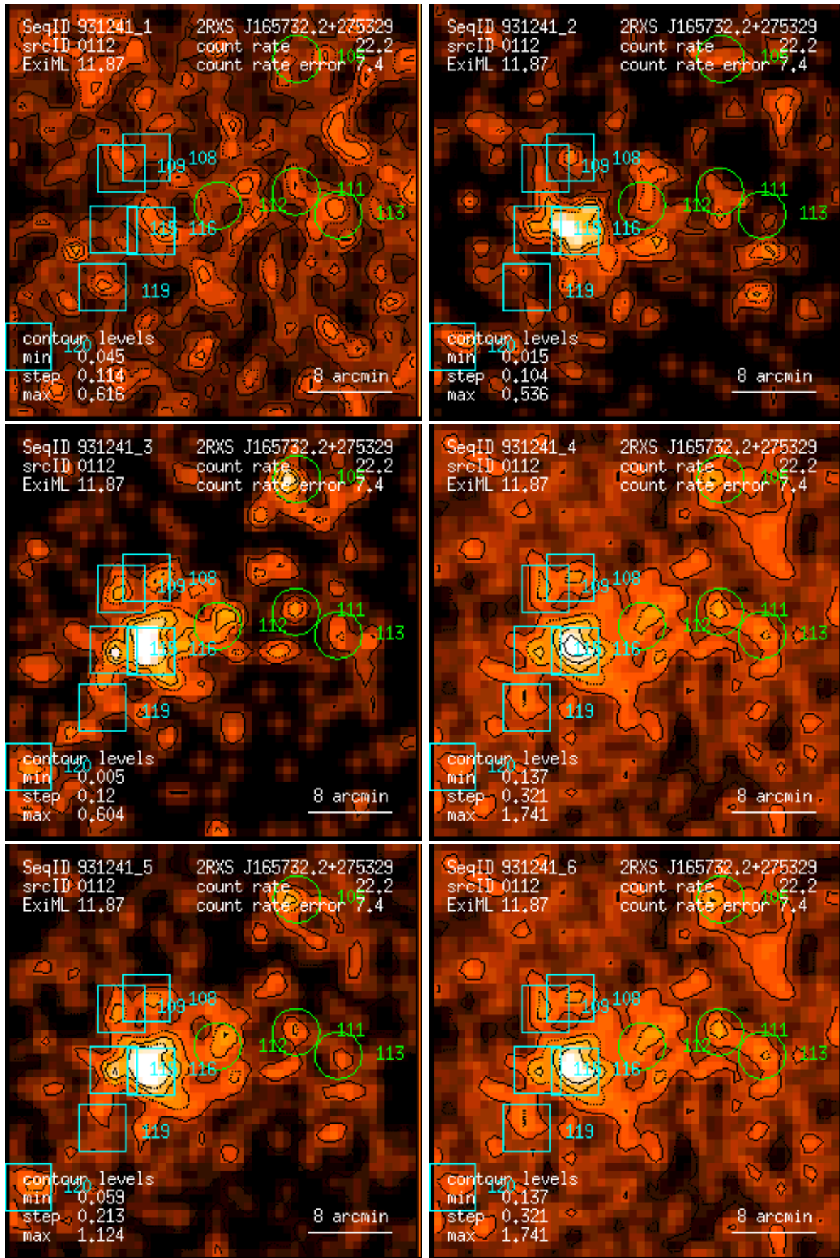
Figure 112: RASS 931241: detection 0112: band rate images, Gaussian filter: (1) PSPC channels 11 – 41, (2) 52 – 90, (3) 91 – 201, (4) 11 – 235, (5) 52 – 201, (6) 11 – 201. Broad band rates in counts/ks. Band rate contour levels in counts/ks/arcmin 2 .
