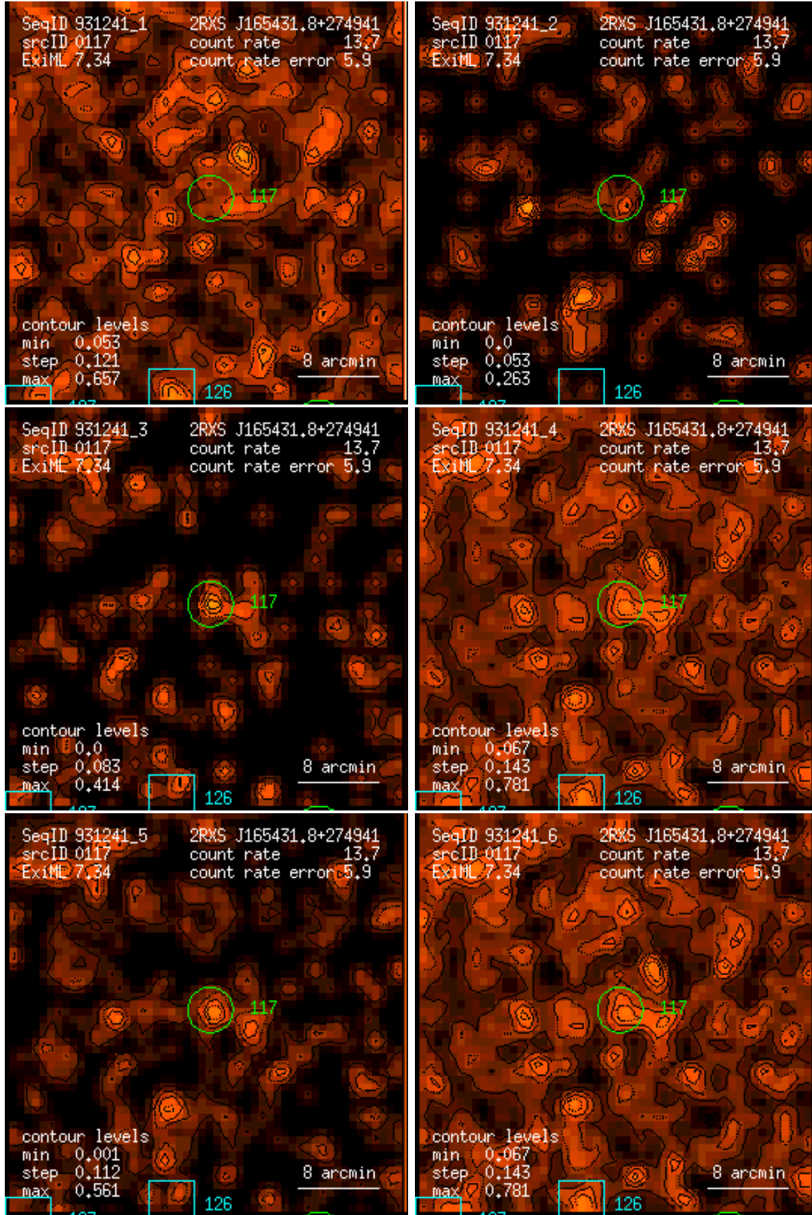
Figure 117: RASS 931241: detection 0117: band rate images, Gaussian filter: (1) PSPC channels 11 – 41, (2) 52 – 90, (3) 91 – 201, (4) 11 – 235, (5) 52 – 201, (6) 11 – 201. Broad band rates in counts/ks. Band rate contour levels in counts/ks/arcmin 2 .
