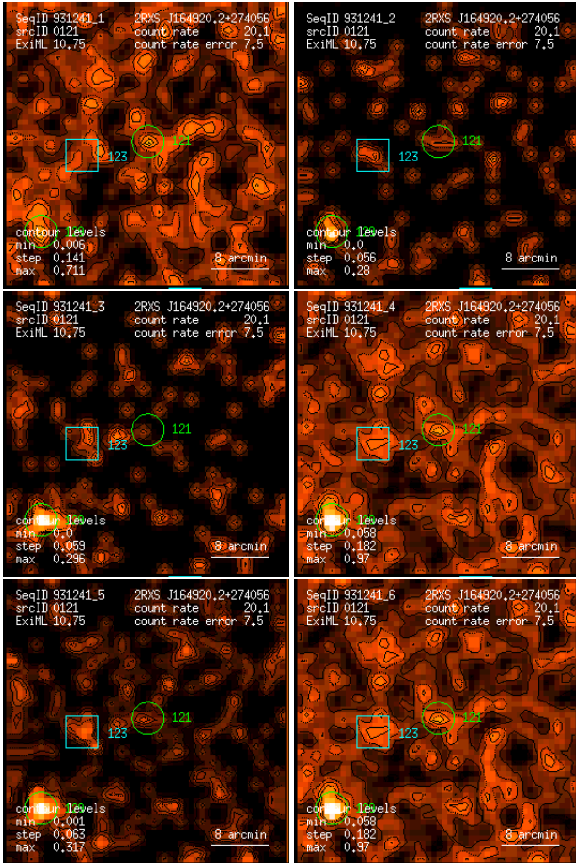
Figure 121: RASS 931241: detection 0121: band rate images, Gaussian filter: (1) PSPC channels 11 – 41, (2) 52 – 90, (3) 91 – 201, (4) 11 – 235, (5) 52 – 201, (6) 11 – 201. Broad band rates in counts/ks. Band rate contour levels in counts/ks/arcmin 2 .
