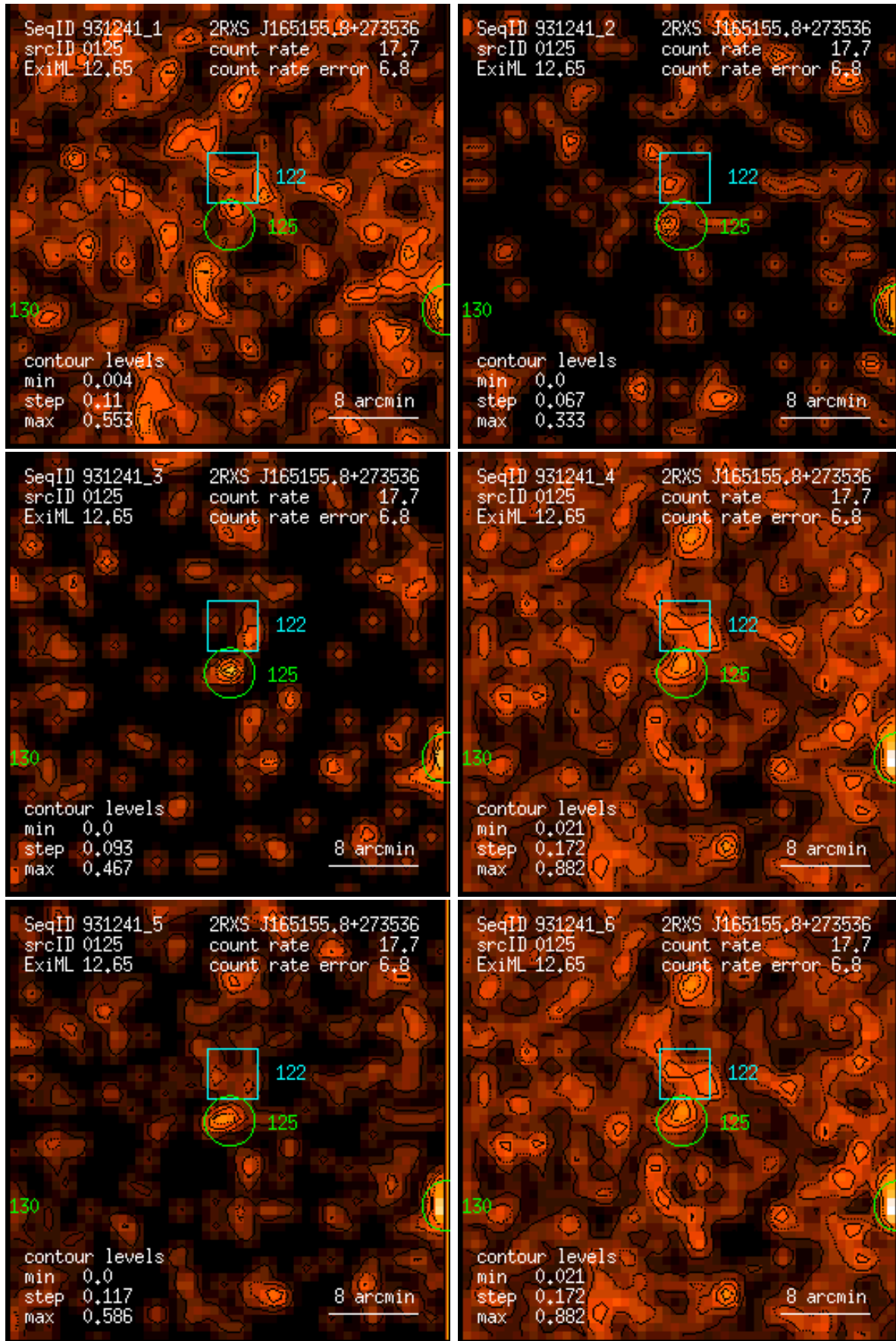
Figure 125: RASS 931241: detection 0125: band rate images, Gaussian filter: (1) PSPC channels 11 – 41, (2) 52 – 90, (3) 91 – 201, (4) 11 – 235, (5) 52 – 201, (6) 11 – 201. Broad band rates in counts/ks. Band rate contour levels in counts/ks/arcmin 2 .
