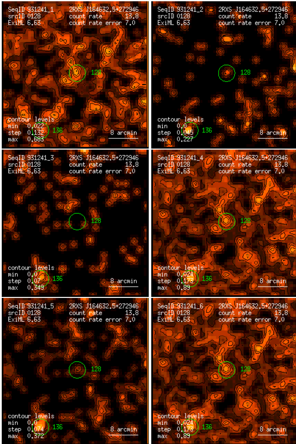
Figure 128: RASS 931241: detection 0128: band rate images, Gaussian filter: (1) PSPC channels 11 – 41, (2) 52 – 90, (3) 91 – 201, (4) 11 – 235, (5) 52 – 201, (6) 11 – 201. Broad band rates in counts/ks. Band rate contour levels in counts/ks/arcmin 2 .
