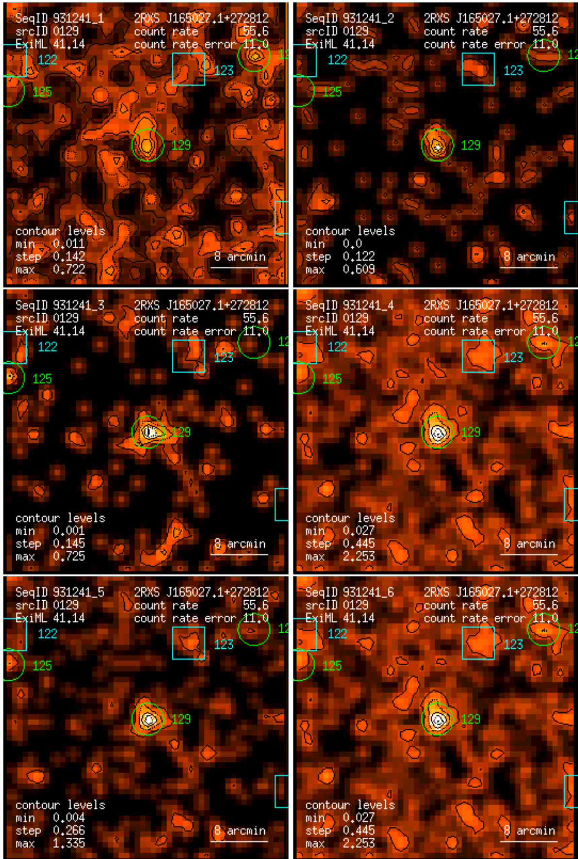
Figure 129: RASS 931241: detection 0129: band rate images, Gaussian filter: (1) PSPC channels 11 – 41, (2) 52 – 90, (3) 91 – 201, (4) 11 – 235, (5) 52 – 201, (6) 11 – 201. Broad band rates in counts/ks. Band rate contour levels in counts/ks/arcmin 2 .
