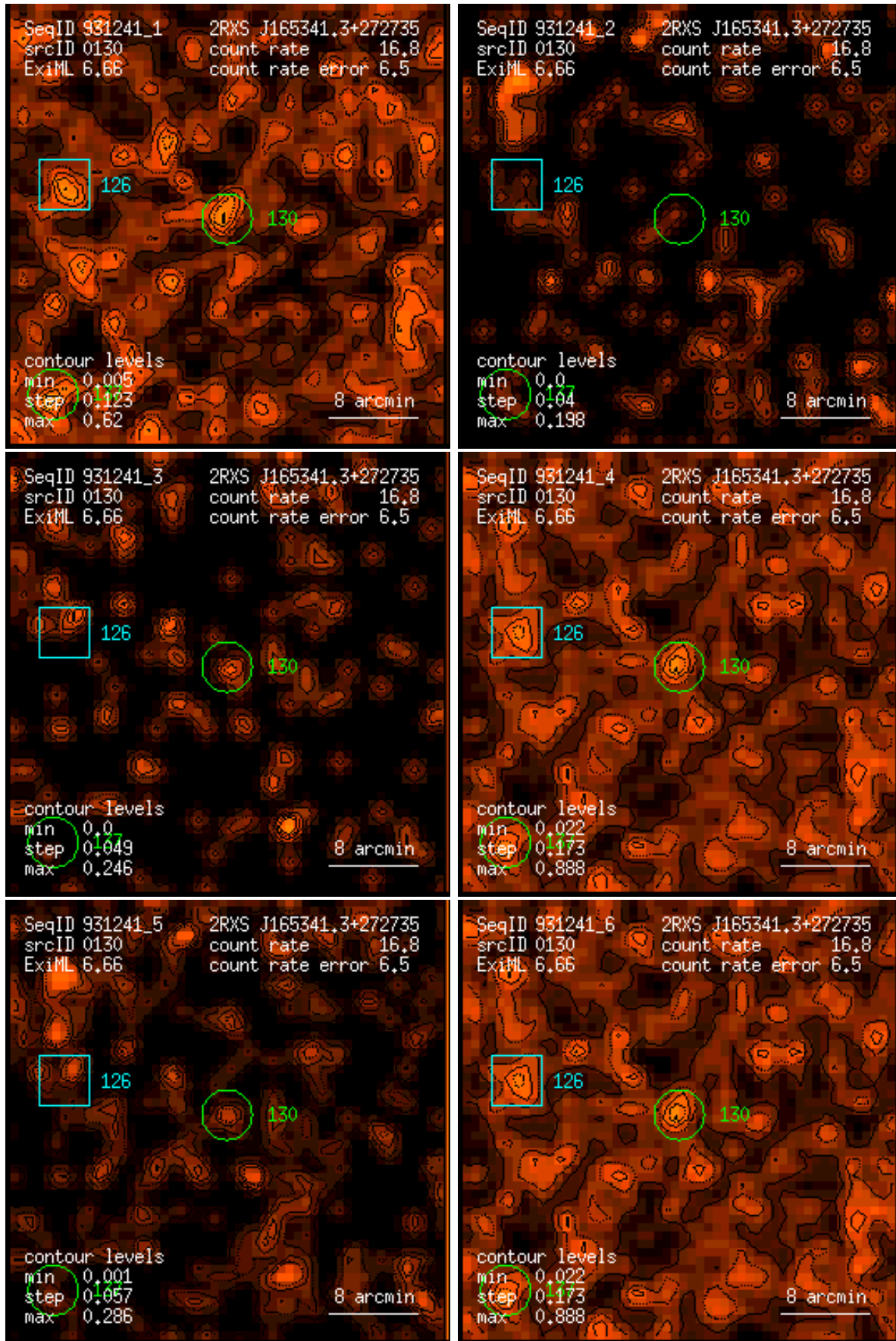
Figure 130: RASS 931241: detection 0130: band rate images, Gaussian filter: (1) PSPC channels 11 – 41, (2) 52 – 90, (3) 91 – 201, (4) 11 – 235, (5) 52 – 201, (6) 11 – 201. Broad band rates in counts/ks. Band rate contour levels in counts/ks/arcmin 2 .
