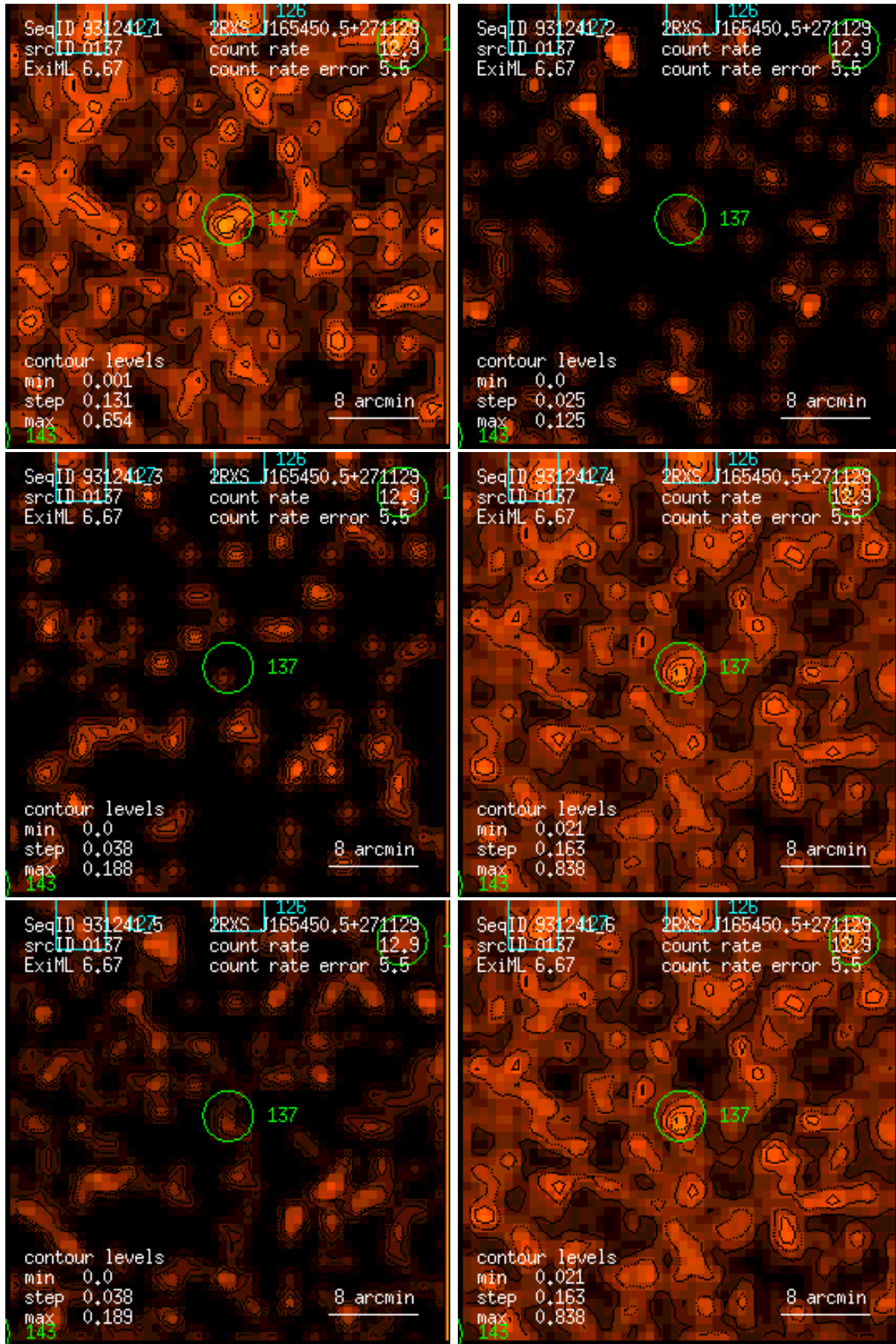
Figure 137: RASS 931241: detection 0137: band rate images, Gaussian filter: (1) PSPC channels 11 – 41, (2) 52 – 90, (3) 91 – 201, (4) 11 – 235, (5) 52 – 201, (6) 11 – 201. Broad band rates in counts/ks. Band rate contour levels in counts/ks/arcmin 2 .
