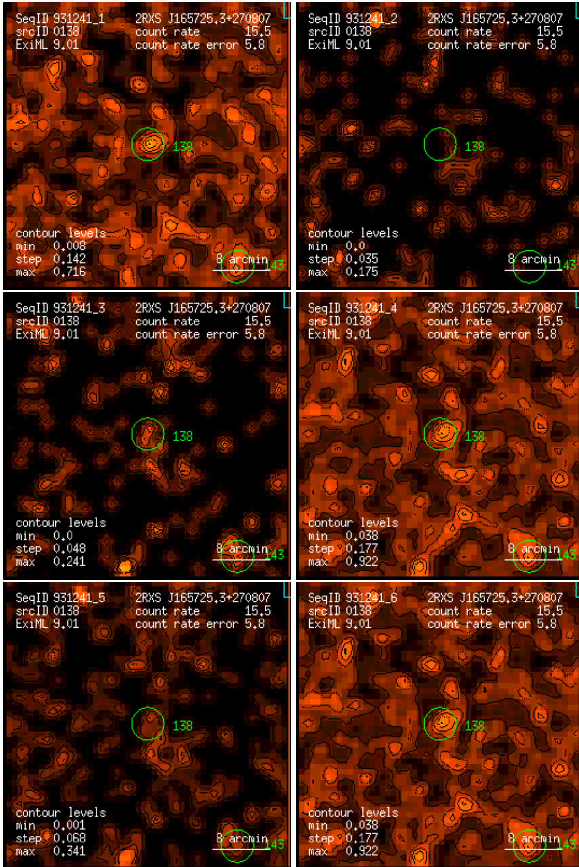
Figure 138: RASS 931241: detection 0138: band rate images, Gaussian filter: (1) PSPC channels 11 – 41, (2) 52 – 90, (3) 91 – 201, (4) 11 – 235, (5) 52 – 201, (6) 11 – 201. Broad band rates in counts/ks. Band rate contour levels in counts/ks/arcmin 2 .
