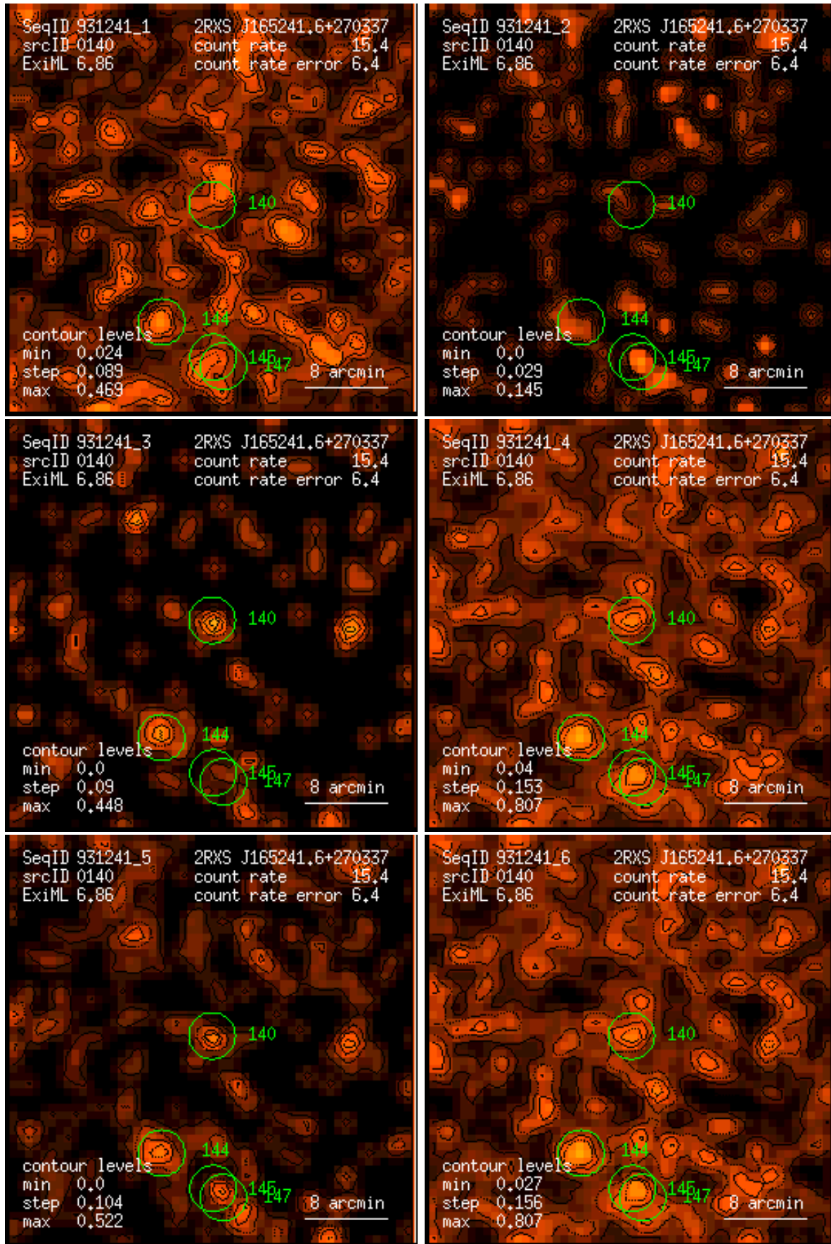
Figure 140: RASS 931241: detection 0140: band rate images, Gaussian filter: (1) PSPC channels 11 – 41, (2) 52 – 90, (3) 91 – 201, (4) 11 – 235, (5) 52 – 201, (6) 11 – 201. Broad band rates in counts/ks. Band rate contour levels in counts/ks/arcmin 2 .
