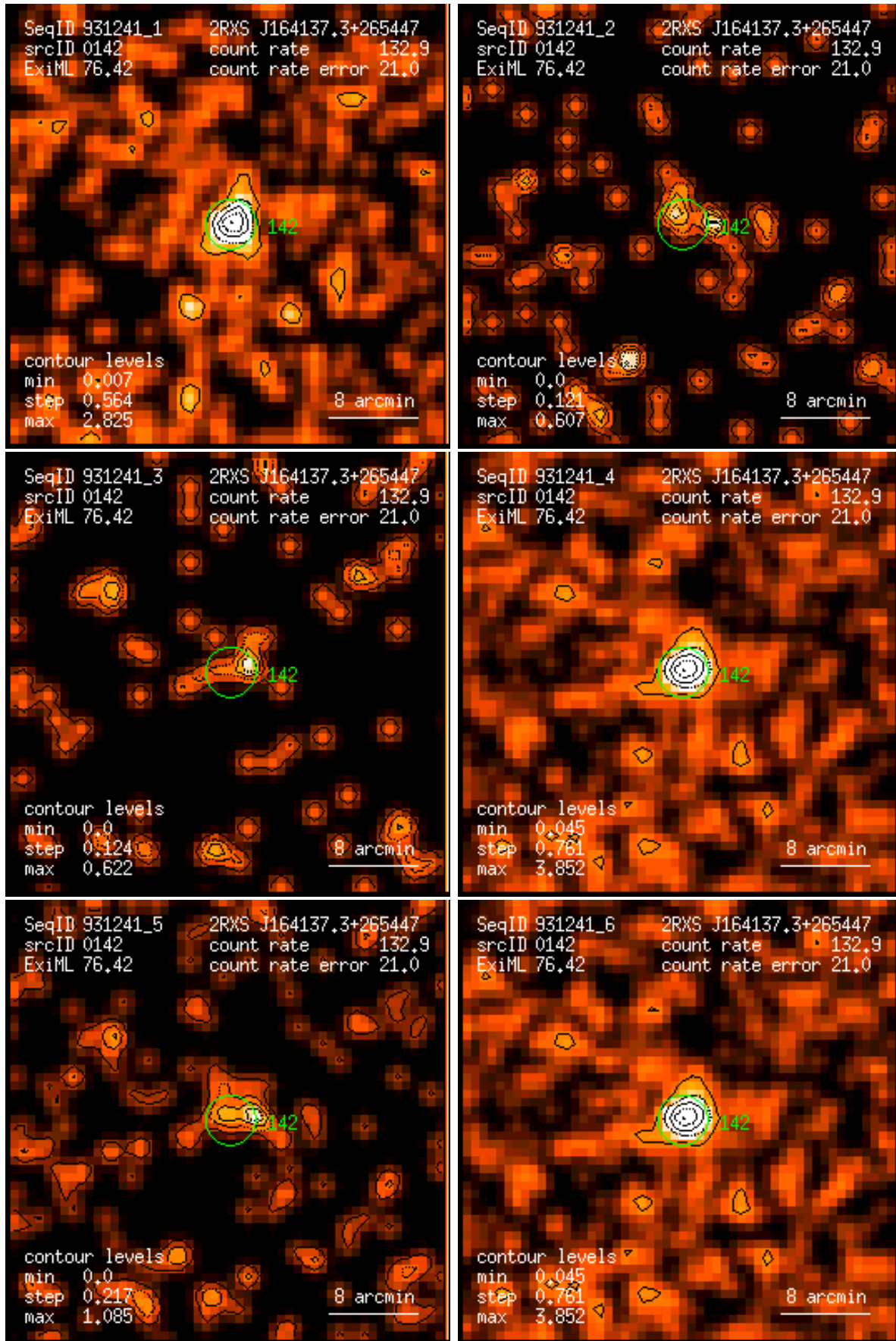
Figure 142: RASS 931241: detection 0142: band rate images, Gaussian filter: (1) PSPC channels 11 – 41, (2) 52 – 90, (3) 91 – 201, (4) 11 – 235, (5) 52 – 201, (6) 11 – 201. Broad band rates in counts/ks. Band rate contour levels in counts/ks/arcmin 2 .
