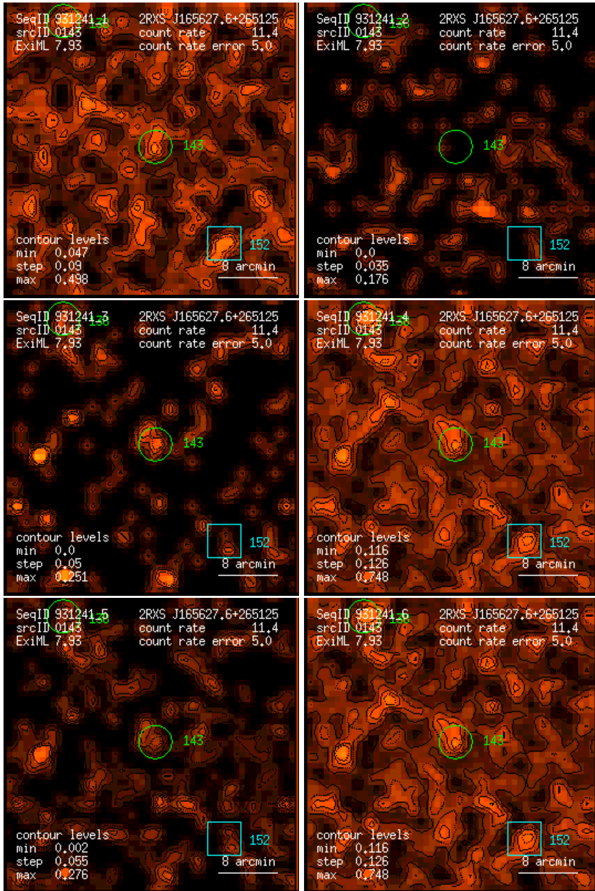
Figure 143: RASS 931241: detection 0143: band rate images, Gaussian filter: (1) PSPC channels 11 – 41, (2) 52 – 90, (3) 91 – 201, (4) 11 – 235, (5) 52 – 201, (6) 11 – 201. Broad band rates in counts/ks. Band rate contour levels in counts/ks/arcmin 2 .
