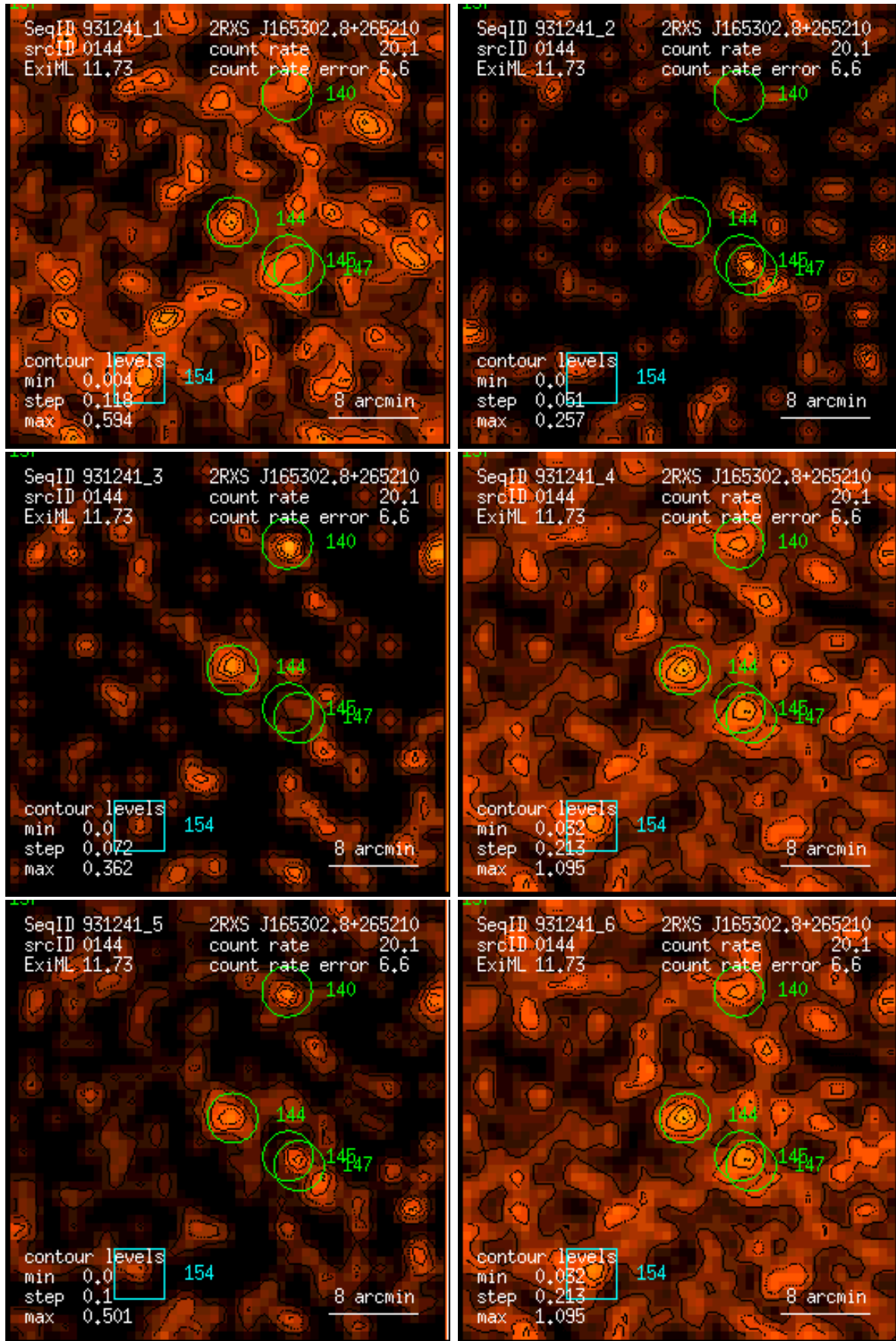
Figure 144: RASS 931241: detection 0144: band rate images, Gaussian filter: (1) PSPC channels 11 – 41, (2) 52 – 90, (3) 91 – 201, (4) 11 – 235, (5) 52 – 201, (6) 11 – 201. Broad band rates in counts/ks. Band rate contour levels in counts/ks/arcmin 2 .
