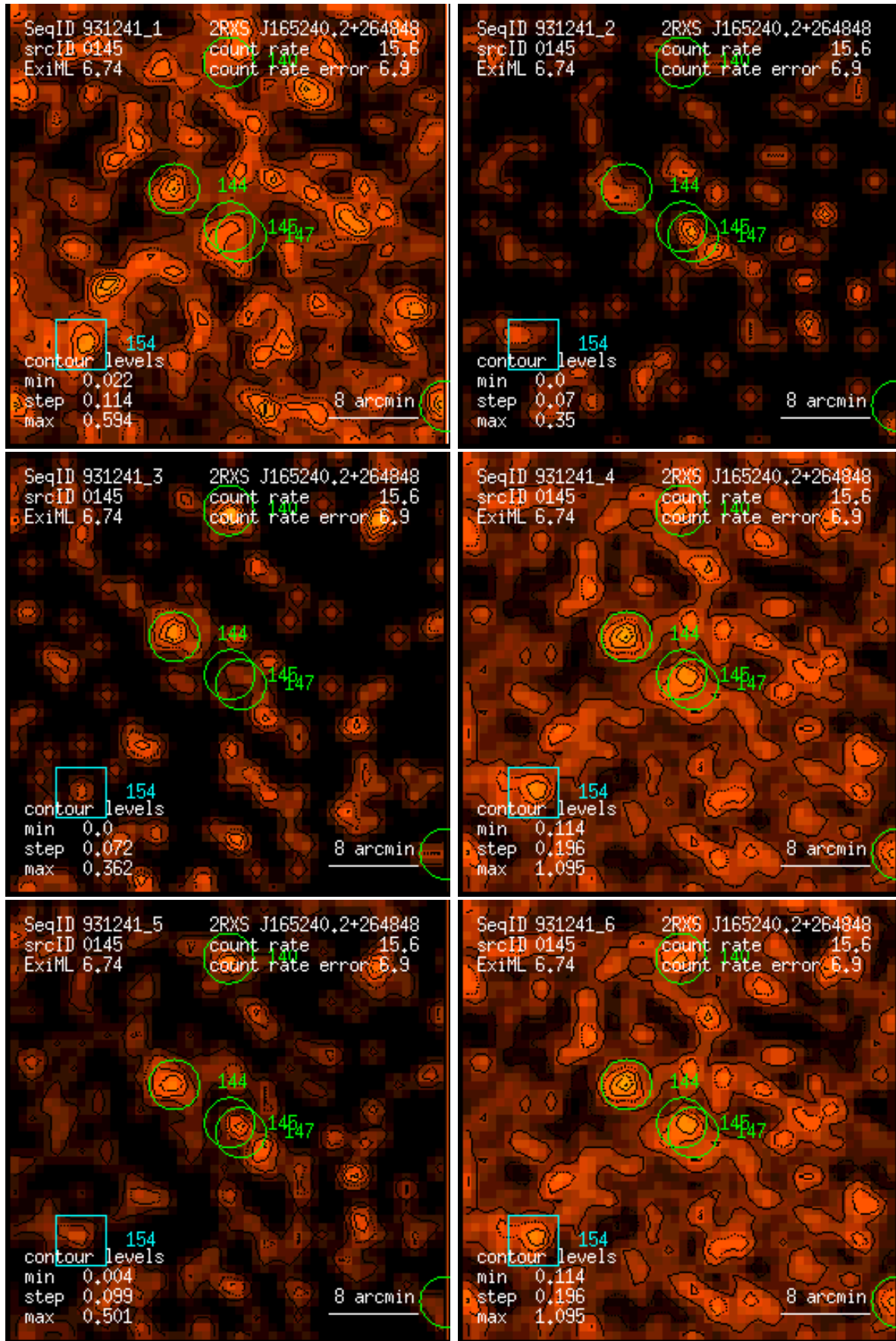
Figure 145: RASS 931241: detection 0145: band rate images, Gaussian filter: (1) PSPC channels 11 – 41, (2) 52 – 90, (3) 91 – 201, (4) 11 – 235, (5) 52 – 201, (6) 11 – 201. Broad band rates in counts/ks. Band rate contour levels in counts/ks/arcmin 2 .
