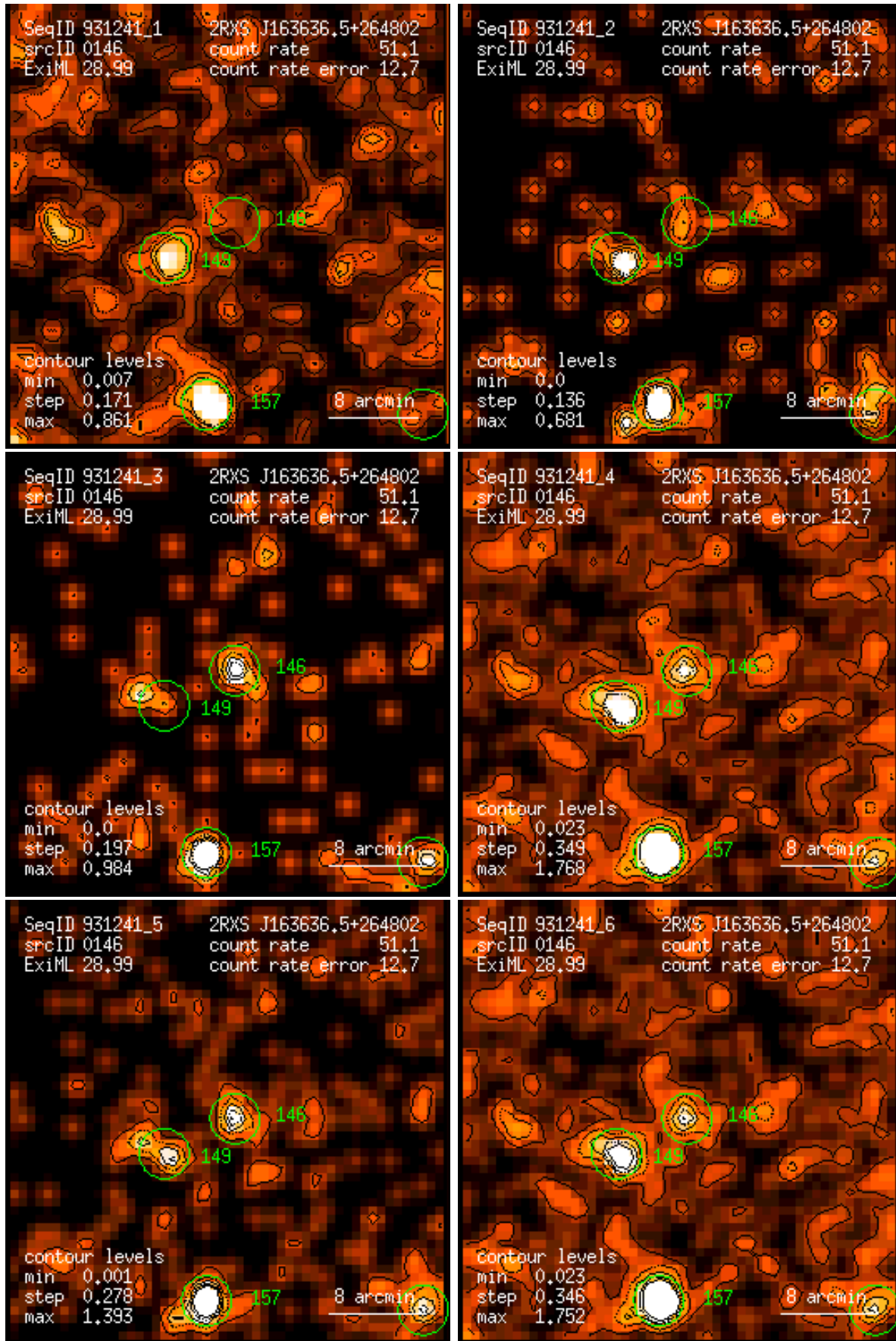
Figure 146: RASS 931241: detection 0146: band rate images, Gaussian filter: (1) PSPC channels 11 – 41, (2) 52 – 90, (3) 91 – 201, (4) 11 – 235, (5) 52 – 201, (6) 11 – 201. Broad band rates in counts/ks. Band rate contour levels in counts/ks/arcmin 2 .
