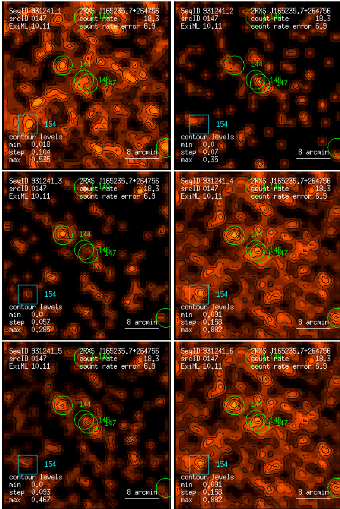
Figure 147: RASS 931241: detection 0147: band rate images, Gaussian filter: (1) PSPC channels 11 – 41, (2) 52 – 90, (3) 91 – 201, (4) 11 – 235, (5) 52 – 201, (6) 11 – 201. Broad band rates in counts/ks. Band rate contour levels in counts/ks/arcmin 2 .
