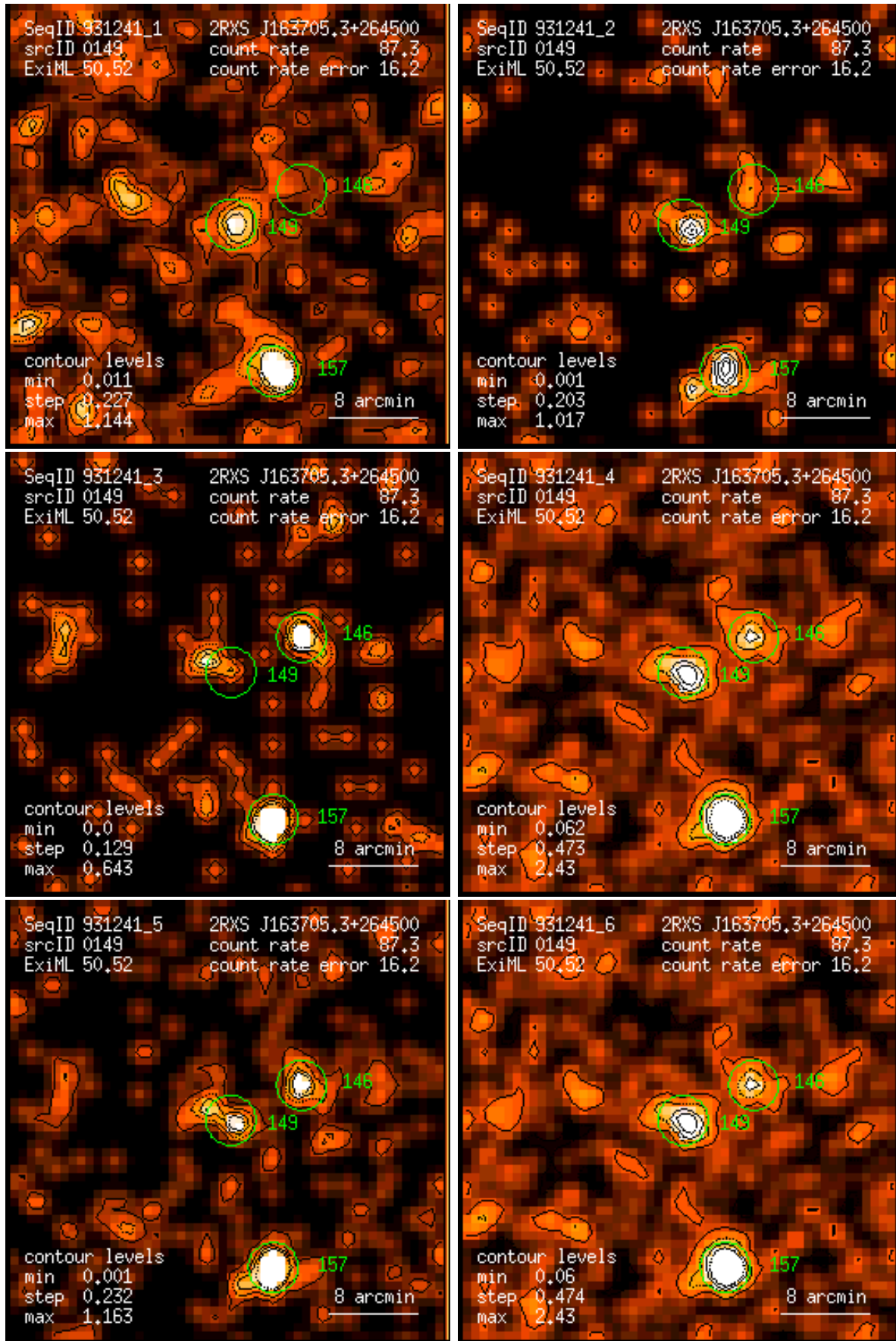
Figure 149: RASS 931241: detection 0149: band rate images, Gaussian filter: (1) PSPC channels 11 – 41, (2) 52 – 90, (3) 91 – 201, (4) 11 – 235, (5) 52 – 201, (6) 11 – 201. Broad band rates in counts/ks. Band rate contour levels in counts/ks/arcmin 2 .
