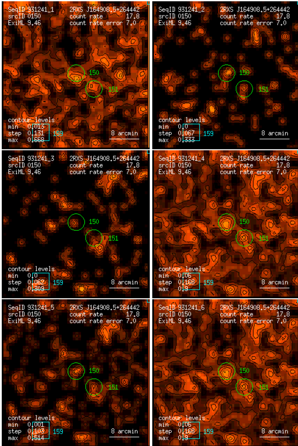
Figure 150: RASS 931241: detection 0150: band rate images, Gaussian filter: (1) PSPC channels 11 – 41, (2) 52 – 90, (3) 91 – 201, (4) 11 – 235, (5) 52 – 201, (6) 11 – 201. Broad band rates in counts/ks. Band rate contour levels in counts/ks/arcmin 2 .
